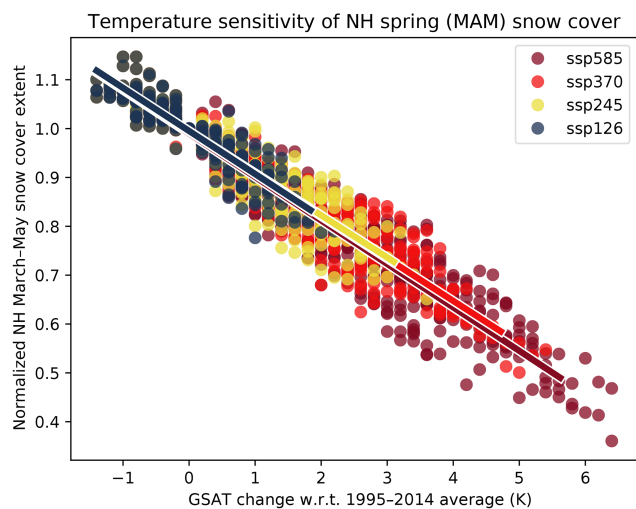
Figure 9. Spring (March to May) NH snow cover extent against GSAT (relative to the 1995–2014 average) for the CMIP6 Tier 1 scenarios (SSP1-2.6, SSP2-4.5, SSP3-7.0, and SSP5-8.5), with linear regressions. Each data point represents the average snow extent from one CMIP6 simulation (first ensemble member for each available model). The average is taken over all pentads from the given simulation which fall into the given temperature bin.
