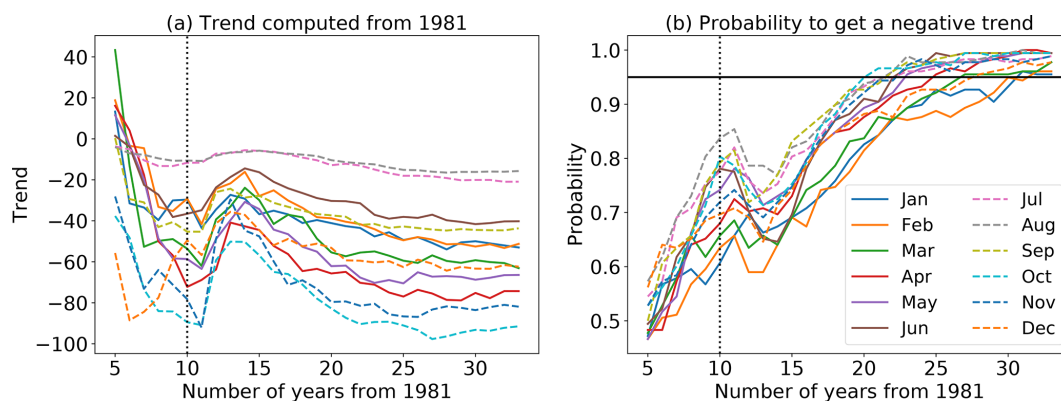
Figure 7. (a) Northern Hemisphere monthly trends of snow extent in CMIP6 models over 1981–2014 computed with 178 members from 21 CMIP6 models as a function of the number of years from 1981 and starting from a 5-year time series. (b) Probability of negative monthly trends estimated from the full ensemble members. The horizontal bar highlights a probability of 95 %, and the vertical bars correspond to the year of the Pinatubo eruption.
