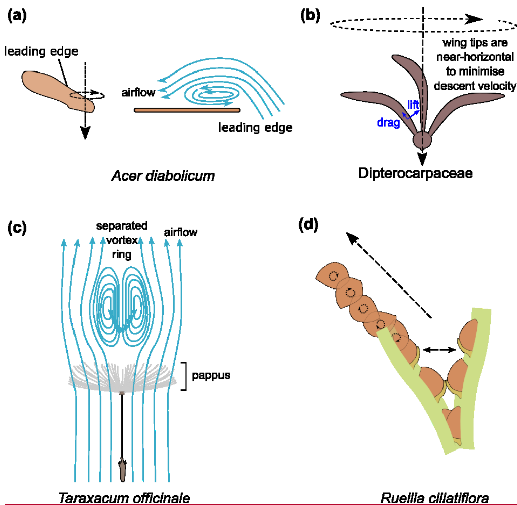
Figure 1. Mechanical mechanisms of dispersal. (a) schematic of a maple samara illustrating the direction of autorotation and descent, and the airflow around a cross section of the samara forming a leading edge vortex, (b) schematic of a typical Dipterocarpaceae diaspore illustrating the rotating motion and direction of descent during flight with blue arrows representing lift and drag forces acting on a wing segment, (c) schematic of a dandelion diaspore illustrating the streamlines of airflow through and around the pappus, (d) schematic of Ruellia ciliatiflora explosive seed ejection demonstrating backspin induced by the launch orientation.
