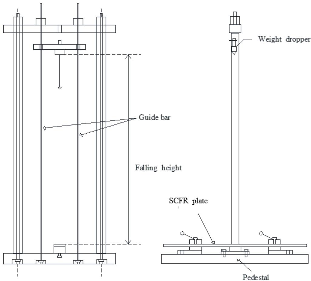
Figure 2. The drop hammer impact device.
