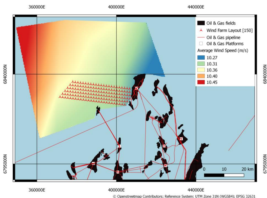
Figure 3 Scaled N8 area wind resource and the chosen layout for the 1.5 GW windfarm with staggered configuration.
