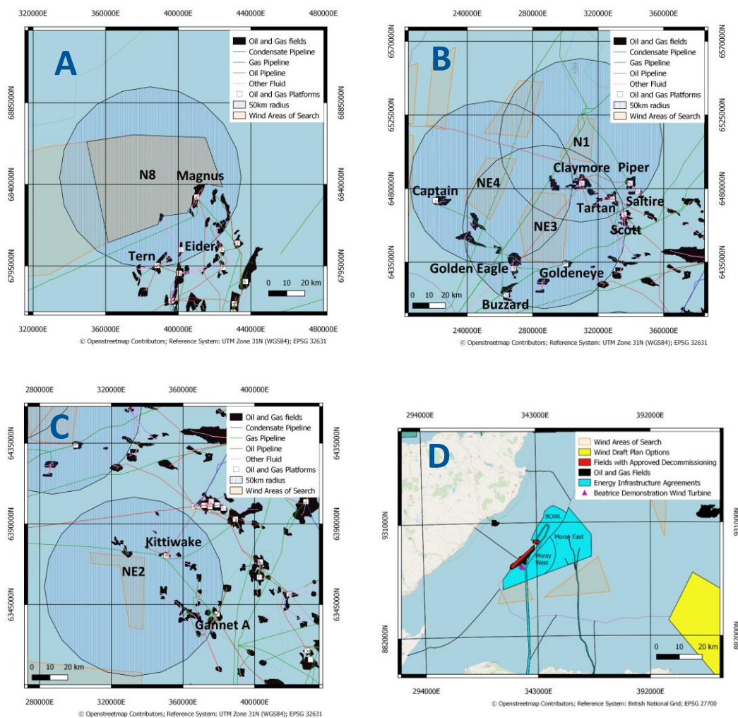
Figure 2 Close up maps of identified areas for offshore hydrogen production around Scotland showing oil and gas infrastructure within 50km radius from wind AoS.
