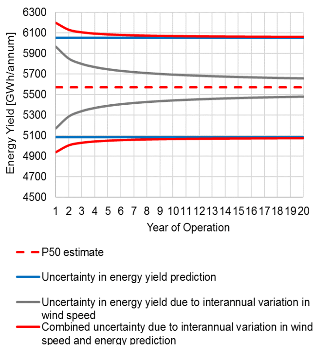
Figure 4 The uncertainty of the energy yield changing with the number of years of the windfarm in operation.
