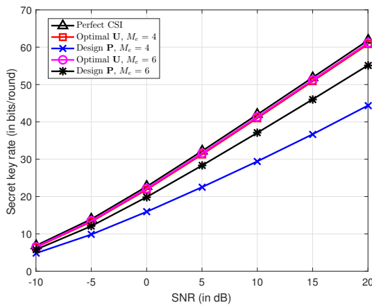
Fig. 4. Secret key rate comparison for one UT.
