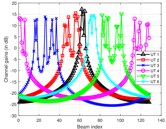
Fig. 5. Multi-user channel gains distribution in the beam domain.
