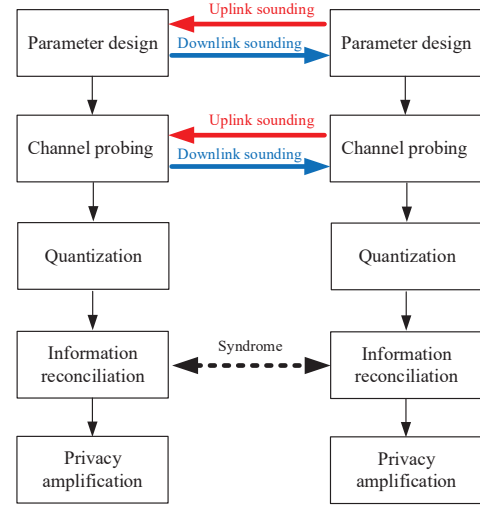
Fig. 2. Flow diagram of CDR based secret key generation scheme.
