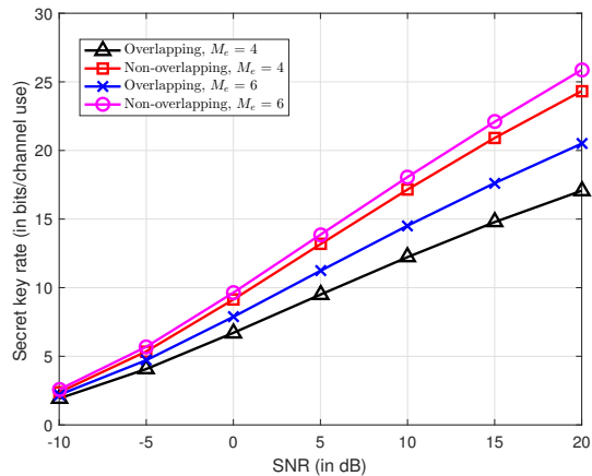
Fig. 8. Unit secret key rate comparison of overlapping and non-overlapping beams.
