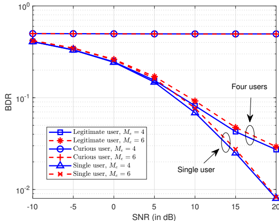
Fig. 10. BDR comparison for legitimate and curious UTs.
