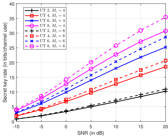
Fig. 6. Secret key rate comparison for different number of UTs.
