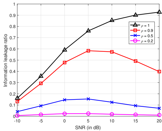
Fig. 9. Information leakage ratio with different correlation coefficients.
