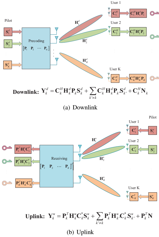
Fig. 3. Channel probing in secret key generation scheme.
