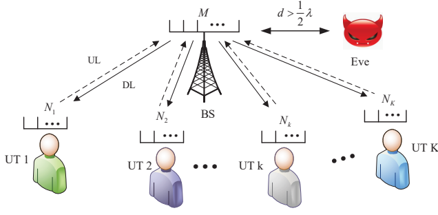
Fig. 1. System model of multi-user secret key generation.
