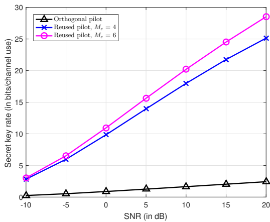
Fig. 7. Unit secret key rate comparison for multiple UTs of orthogonal pilot and reused pilot.
