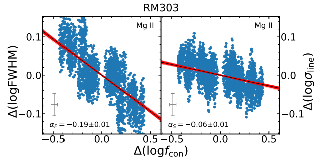
Figure 7. The \Delta \log W - \Delta \log L correlation of RM303 for Mg II during the 2014-2017 observations of SDSS-RM.
