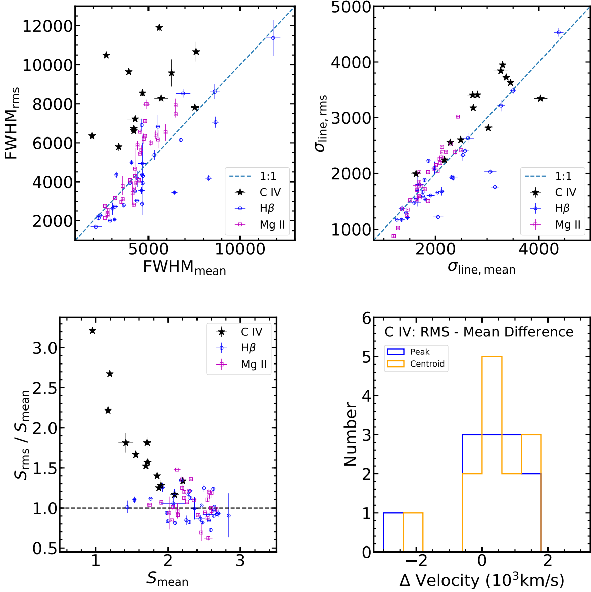
Figure 14. rms and mean profile comparisons for H \beta , Mg II, and C IV. The upper two panels are the comparison for FWHM and \sigma_{\text{line}} , respectively. The lower two panels are line shape ratio comparison and centroid velocity difference distribution, respectively. C IV shows noticeable worse correlation between the rms and mean widths than H \beta and Mg II, mainly due to the non-reverberating core component (see text for details). This non-varying core C IV component has less impact on \sigma_{\text{line}} than on FWHM.
