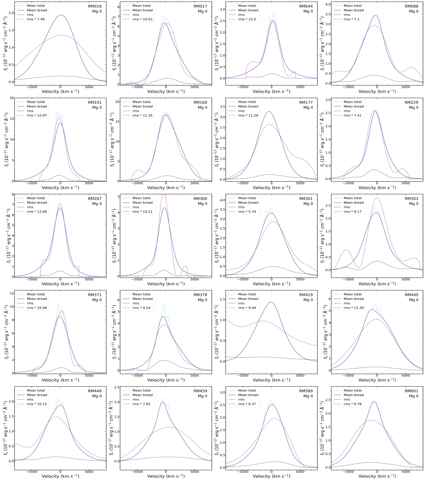
Figure 23. Same as Figure 21 but for Mg II.
