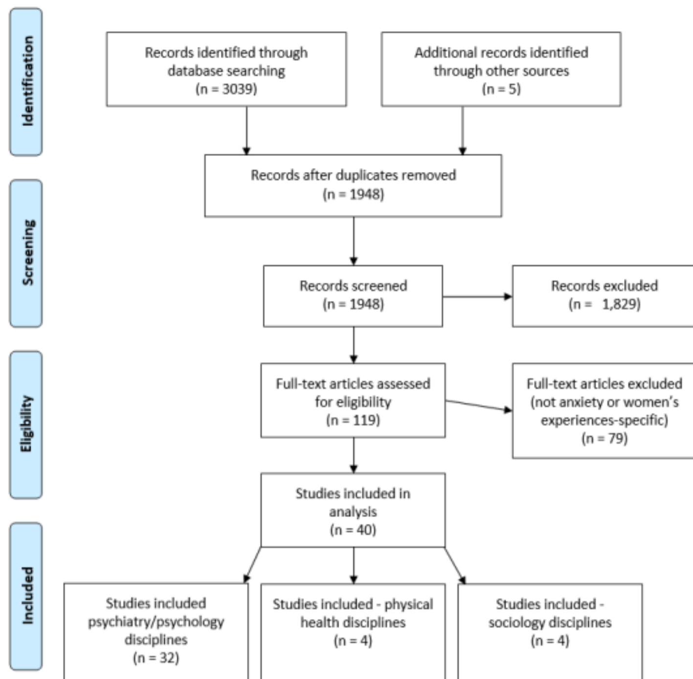
FIGURE 2: PRISMA diagram
