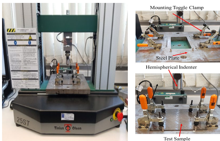
Fig. 1 Low velocity impact test set-up
