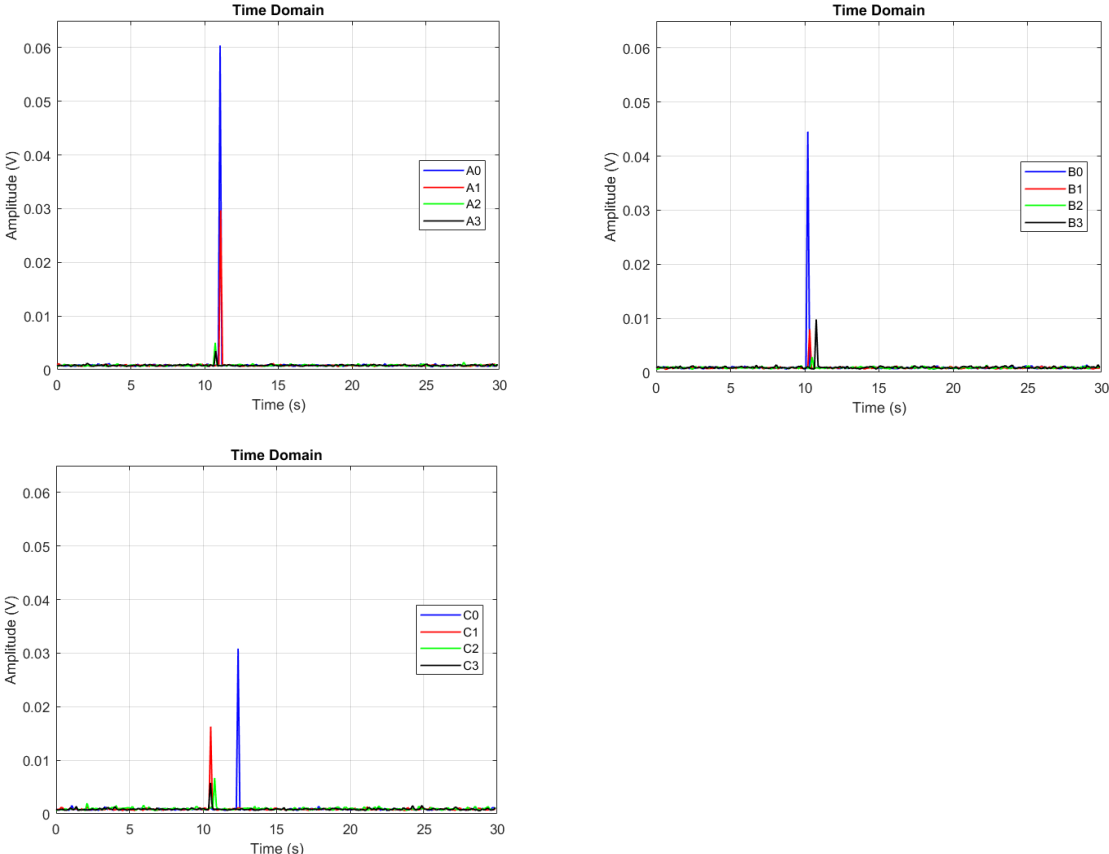
Fig. 4 Time domain AE response for test samples A(0-3), B(0-3) and C(0-3)
