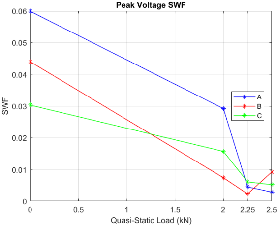
Fig. 5 Peak voltage SWF analysis for test samples A(0-3), B(0-3) and C(0-3)
