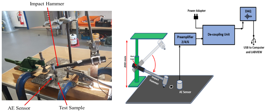
Fig. 3 Vibro-Acoustic test set-up
