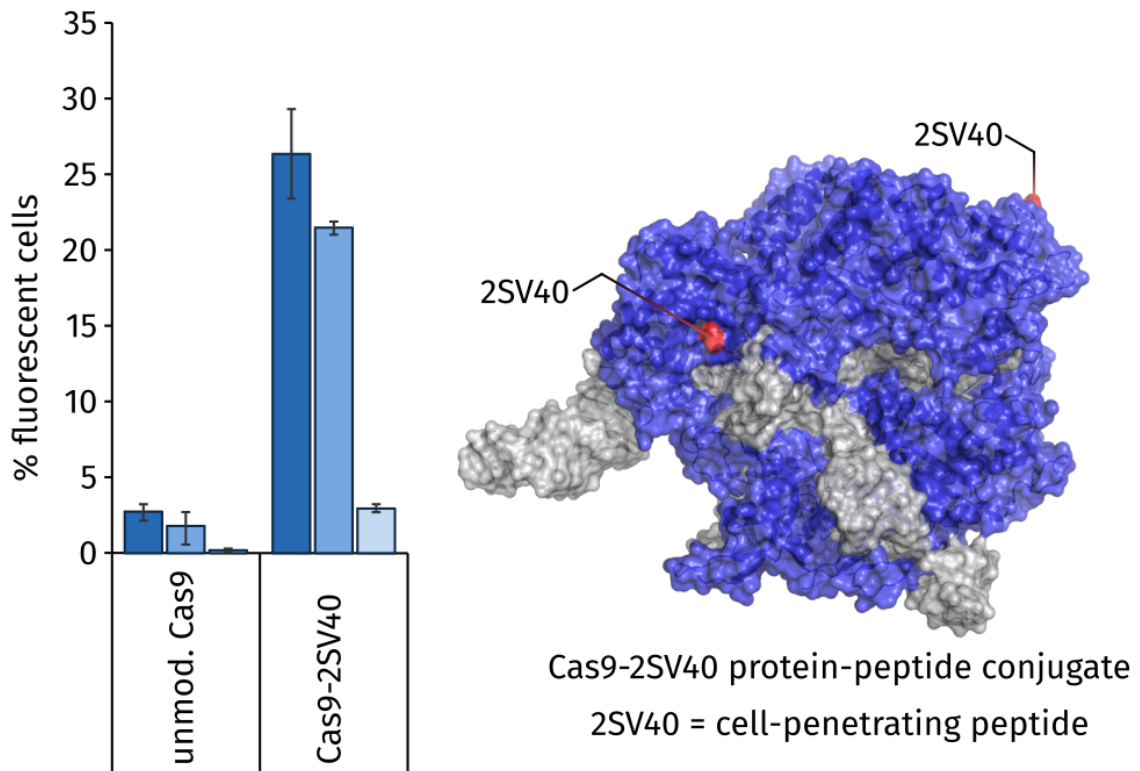
Fig. 2. Left: Improved cellular delivery of Cas9-2SV40 protein-peptide conjugate relative to an unmodified control, assayed by cell fluorescence. Reproduced with permission from ref 1.
