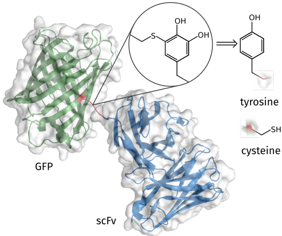
Fig 1. Protein-protein conjugate of the green fluorescent protein (GFP) and an antibody fragment (scFv). The linkage arises from the coupling of a tyrosine and cysteine residue, mediated by the tyrosinase enzyme.
