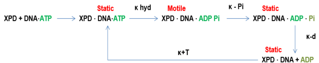
Figure 5.14 Schematic model for the interaction of XPD and double stranded DNA and ATP hydrolysis.
