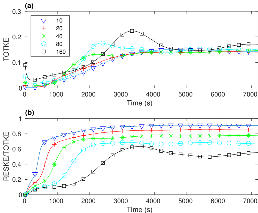
Figure 2. Time series of (a) total (resolved plus sub-filter) kinetic energy (TOTKE) in m^2s^{-2} and (b) the ratio of resolved kinetic energy (RESKE) to total kinetic energy, for CBL1 simulations. Each line is for a simulation with a different grid length, the values in m being indicated in the inset.
