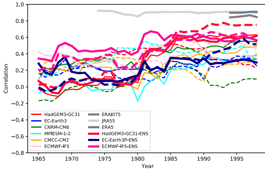
FIG. 11. Correlation of TRACK ACE 925 from models and reanalyses for North Atlantic tropical cyclone variability against Observed ACE as a function of time, using a moving 30-yr period centered on the year shown. The dashed lines are for lower resolution, and solid lines are for higher-resolution models and reanalyses. The “-ENS” lines are for up to three member ensemble means from the available models.
