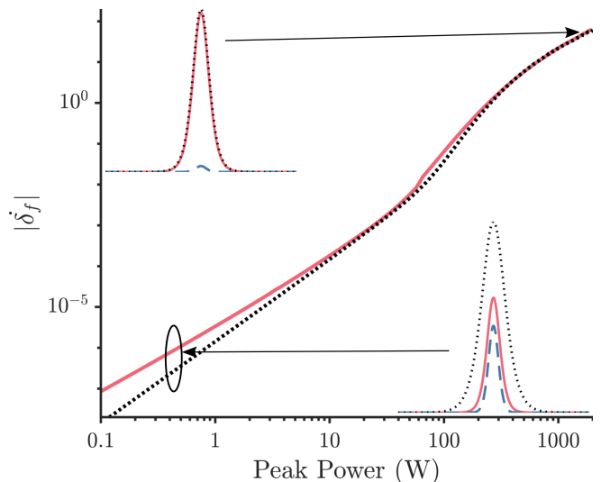
FIG. 3. Rate of frequency shift, \dot{\delta}_f , predicted by Eq. (16) for two-component solitons and Kerr solitons in LN nano-waveguides; shown as solid (red) and dotted (black) curves respectively (for \nu = 0 ). For the two-component solitons we plot the peak power as |A_f|^2 + |A_s|^2 . Insets compare soliton power profiles at high and low powers. FF and SH of the two-component solitons are plotted as solid (red) and dashed (blue) curves respectively. Kerr soliton power profile shown as dotted (black) curve with the same total peak power. We found that \dot{\delta}_s/2 very closely followed the same trend as \dot{\delta}_f for the two-component soliton in this case.
