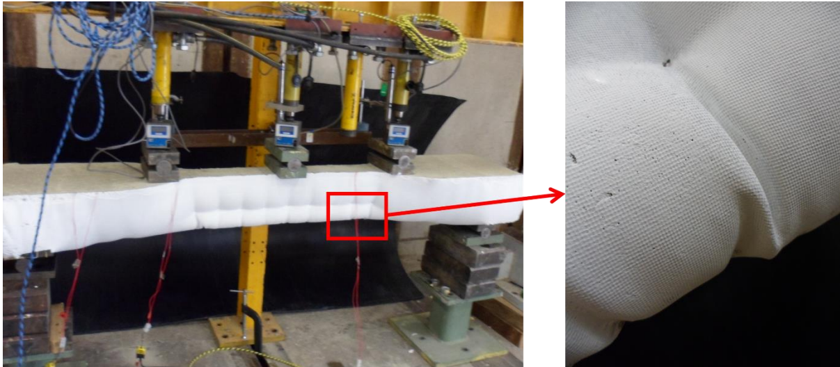
Figure 10 Undesirable fabric wrinkling in tensile reinforcement cover zone
