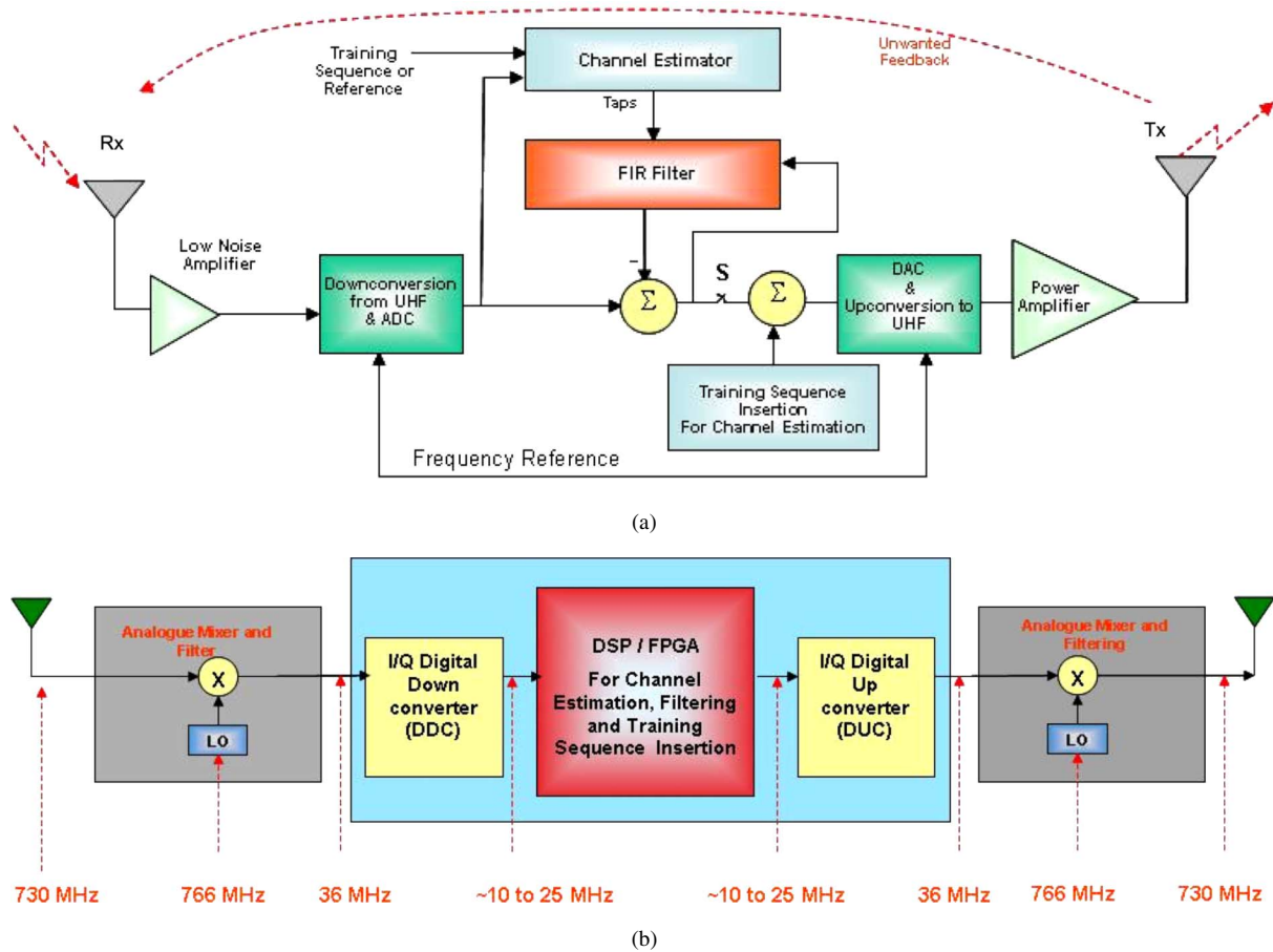
Fig. 1. (a) Block diagram of the proposed on-channel repeater with echo canceller. (b) Block diagram of the repeater system showing the main filtering stages with an example of a UHF channel at 730 MHz.
