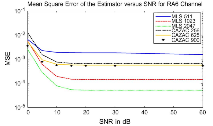
Fig. 9. Comparison of the MSE performance of different training sequences for a rural area channel.
