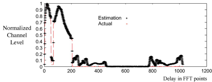
Fig. 8. Comparison of actual and estimated BU12 channel using a CAZAC sequence of length 900 at an SNR of 20 dB.
