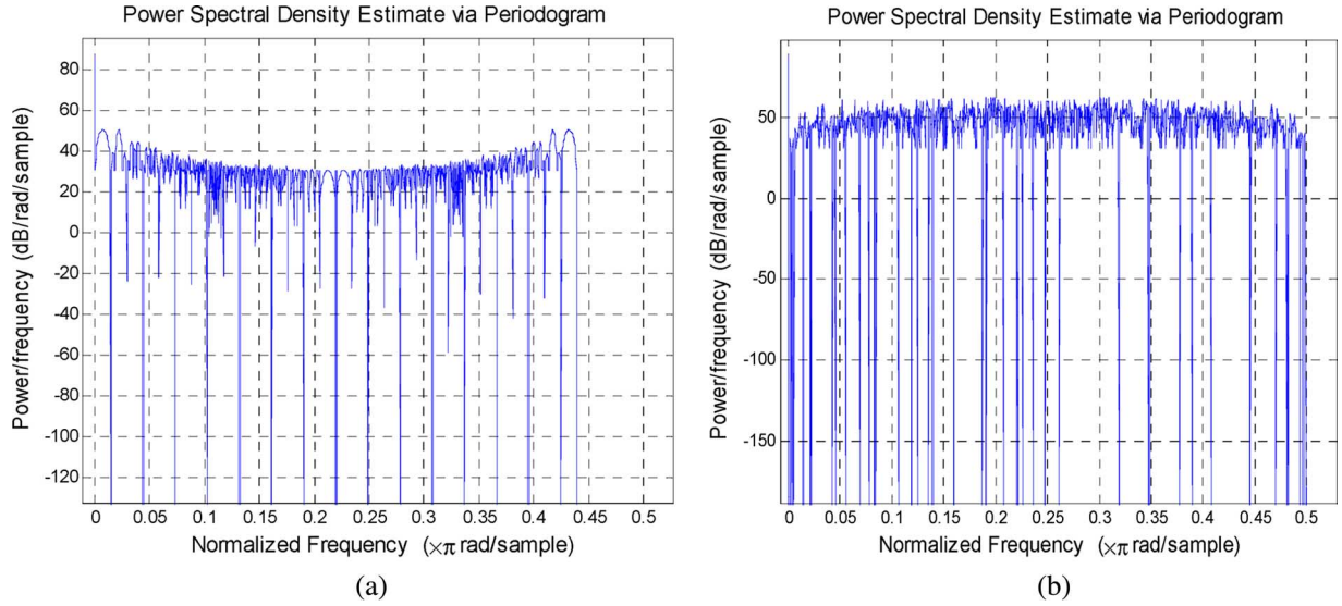
Fig. 6. Simulated Power Spectral Densities of (a) the CAZAC900 and (b) MLS1023 sequences with 4096 FFT points.
