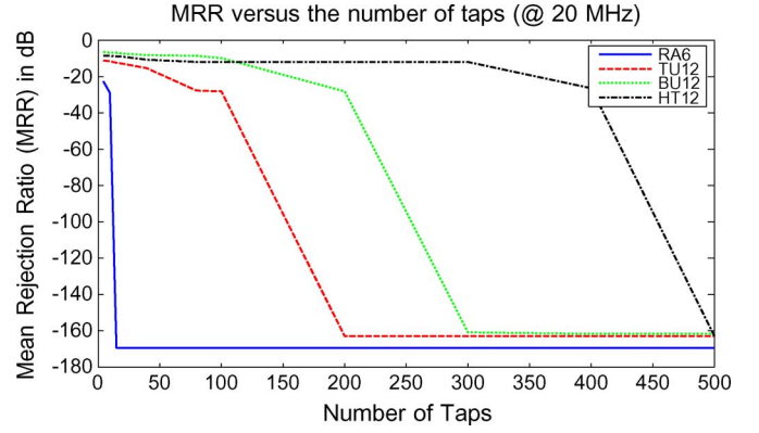
Fig. 3. Expected isolation of the proposed echo canceller versus the number of taps at 20 MHz sampling.
