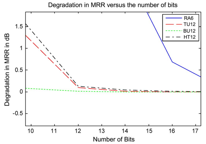
Fig. 4. Expected degradation in the isolation figure caused by the use of fixed point arithmetic.
