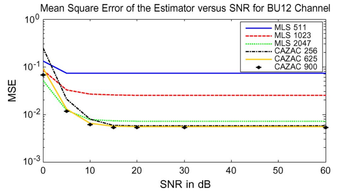
Fig. 10. Comparison of the MSE performance of different training sequences for a bad urban channel.
