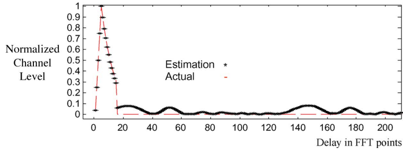
Fig. 7. Comparison of actual and estimated RA6 channel using a CAZAC sequence of length 900 at an SNR of 15 dB.
