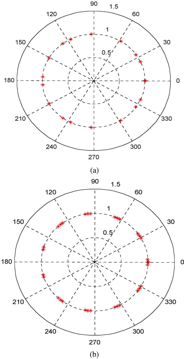
Fig. 5. Roots of unity “R” for CAZAC sequences of length 256 and 900. (a) constellation of the 16 roots of unity for a CAZAC sequence of length 256; (b) constellation of the 30 roots of unity for a CAZAC sequence of length 900.
