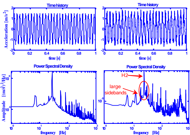
Fig. 5 – Regular and irregular idle vibrations.
