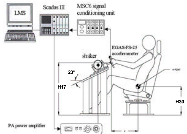
Fig. 6 – Steering vibration simulator.
