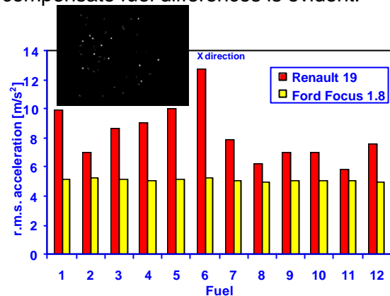
Fig. 2 – Vibration levels at the engine block.
