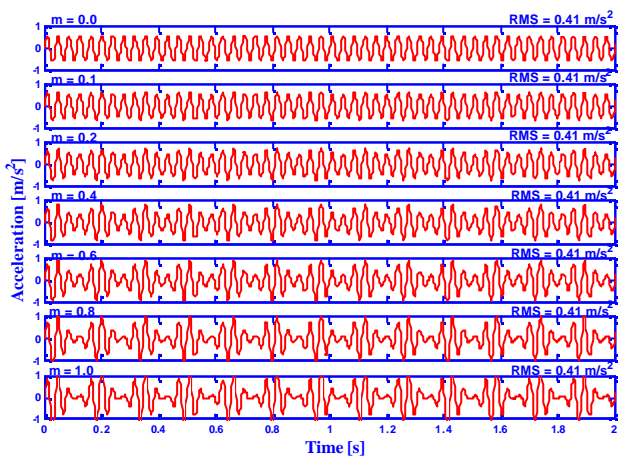
Fig. 7 – Amplitude modulated test stimuli.
