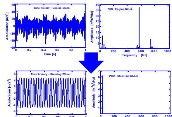
Fig. 4 – Transmission of vibration to wheel.
