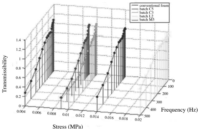
Figure 7. ISO 13753 transmissibility ratios versus frequency and compressive stresses at 10% compressive strain for the different types of foams
