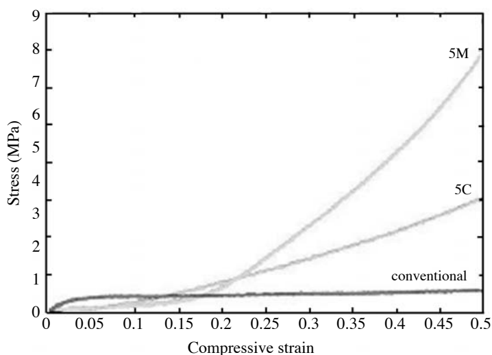
Figure 5. Comparison of compressive stress-strain curves for conventional, types 5C and 5M foams up to 50% of strain
