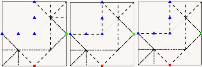
Figure 5: Crease patterns for angle fractions 0.3, 0.5, and 0.8.
