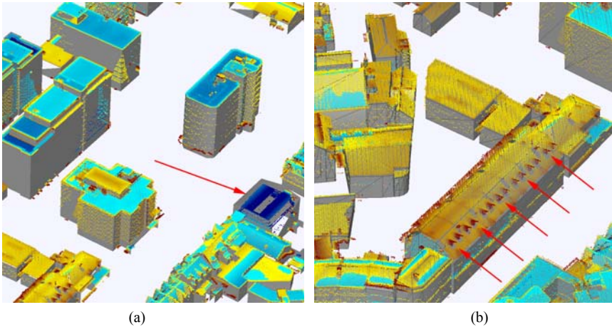
FIG. 9. (a) A zoom-in to the central part of Fig. 8(b), in oblique view. The red arrow shows a building with large differences between the model and the point cloud. (b) A zoom-in to the lower-left part of Fig. 8(b), in oblique view. The missing dormers (indicated by the red arrows) can easily be identified by the LS3D surface matcher. Ordnance Survey © Crown copyright. All rights reserved.
