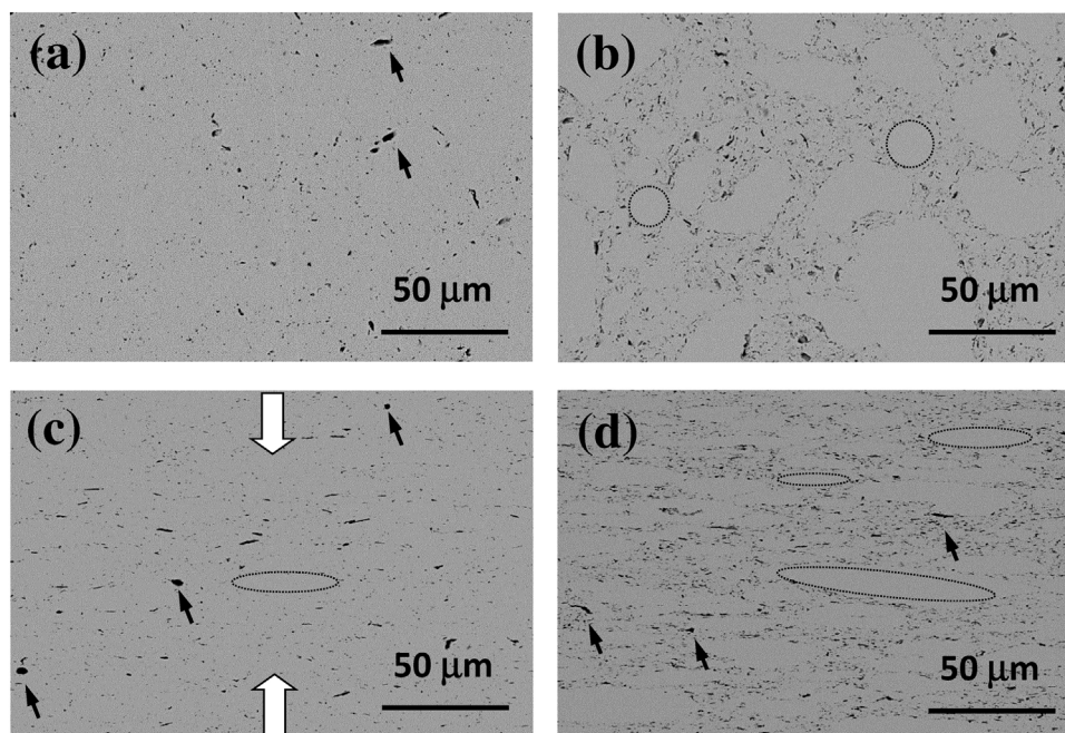
Fig. 3 – Backscattered scanning electron (BSE) microscopy images from the composites i.p. (a, b) and c.s. (c, d) polished surfaces: (a and c) 1 vol%, (b and d) 4 vol% BNNS. Compression axis during SPS is indicated in (c) by arrows.
