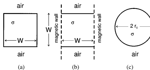
Fig. 1. Cross section of the wires whose internal impedances are compared in Fig. 2. (a) An example structure analyzed in Fig. 6 of the above paper. (b) The same structure with magnetic walls eliminating corner effects. (c) Round wire having the same dc resistance as the previous wires. Dimensions: W = 4.62 mm, r_0 = W/\sqrt{\pi} . Conductivity: \sigma = 5.72 \times 10^7 ( \Omega \cdot m ) -1 .
