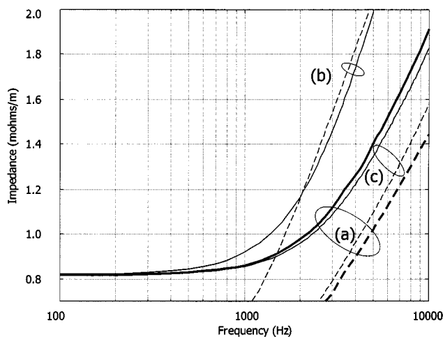
Fig. 2. Internal resistances (solid lines) and reactances (dashed lines) of the wires in Fig. 1. Thick lines correspond to data appearing in Fig. 6 in the above paper for the structure in Fig. 1(a).
