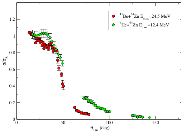
Figure 1: (Color online) Comparison of scattering angular distribution for ^{11}\text{Be} (red circles) and ^6\text{He} (green diamonds) on a ^{64}\text{Zn} target at similar energies with respect to the Coulomb barrier.
