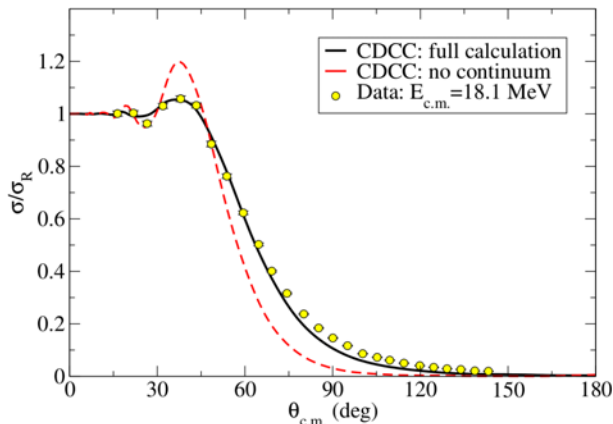
Figure 2: (Color online) Elastic scattering angular distribution for {}^6\text{Li}+{}^{64}\text{Zn} at E_{\text{c.m.}}=18.1 MeV. Symbols are the experimental data, the full line represent the CDCC calculation with full coupling while the dashed line represent the calculation with no-continuum coupling.
