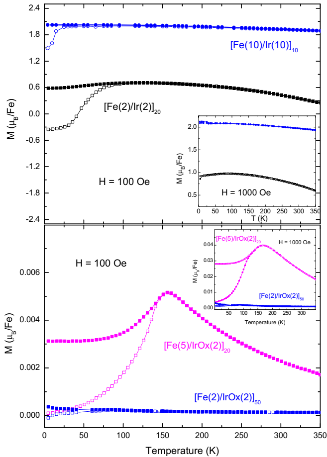
FIG. 9. FC and ZFC magnetothermal curves.
