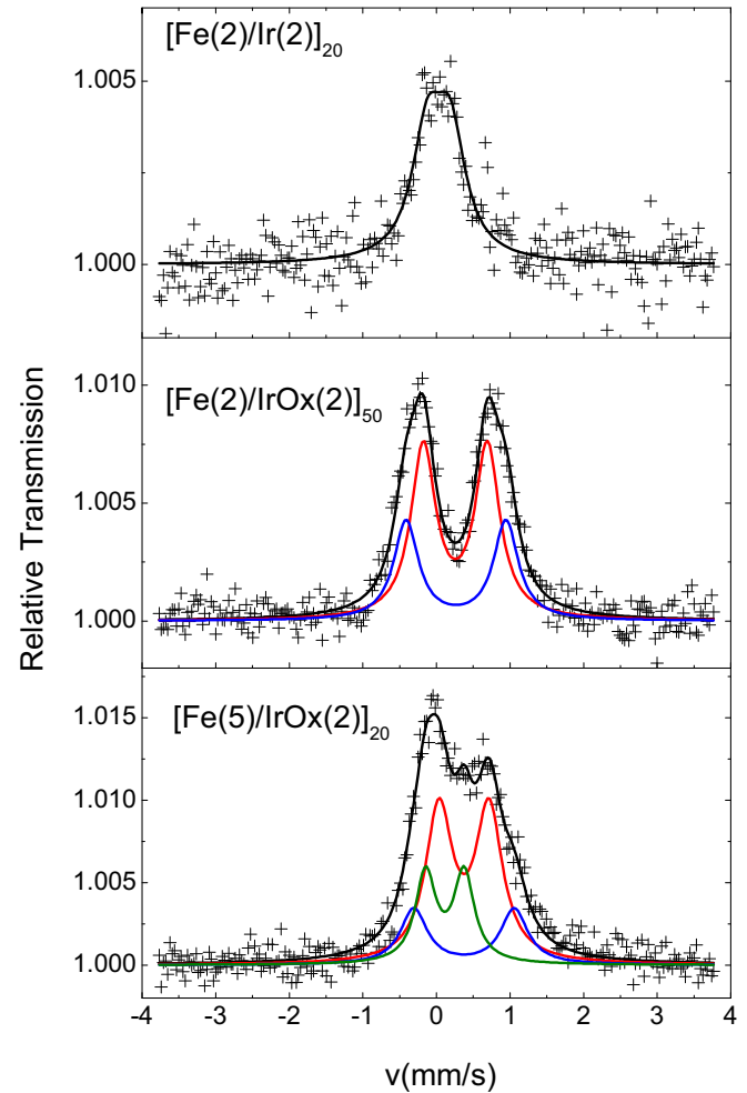
FIG. 10. Mössbauer spectra measured at room temperature. Each panel shows the experimental spectra (+), the overall fit (solid black lines), and the different components: 1 (red), 2 (blue), and 3 (olive) used to fit the experimental spectra.
