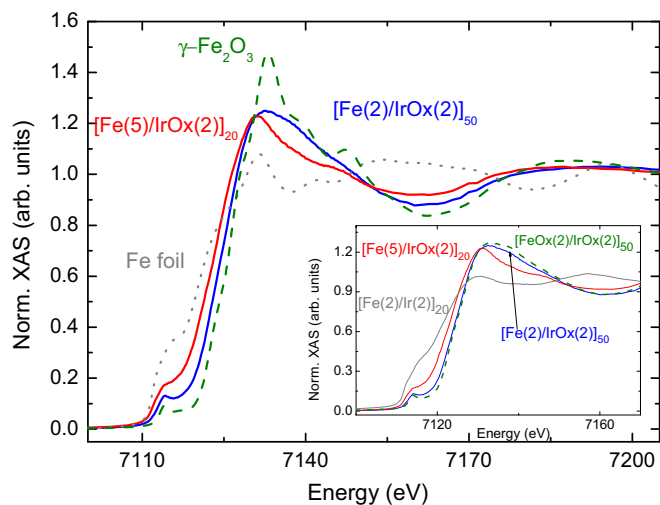
FIG. 5. Fe K-edge XAS spectra of [\text{Fe}(2)/\text{IrOx}(2)]_{50} , [\text{Fe}(5)/\text{IrOx}(2)]_{20} , and bulk \text{Fe}_2\text{O}_3 and Fe foil references.
