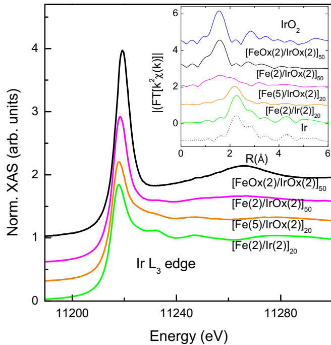
FIG. 7. Comparison of the Ir L_3 -edge XANES spectra. For the sake of clarity the spectra have been vertically shifted. Inset: Fourier transforms ( k^2 weighted, range from 3.1 \text{ \AA}^{-1} to 10 \text{ \AA}^{-1} ) of the EXAFS signals recorded at the Ir L_3 edge. The dotted line corresponds to the simulated spectrum of Ir metal. \text{IrO}_2 was measured in transmission geometry.
