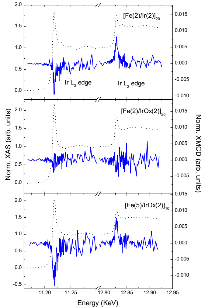
FIG. 11. Normalized XAS and XMCD spectra recorded at the L 2,3 edges of Ir at T = 10 K and H = 3.5 T on three representative samples.
