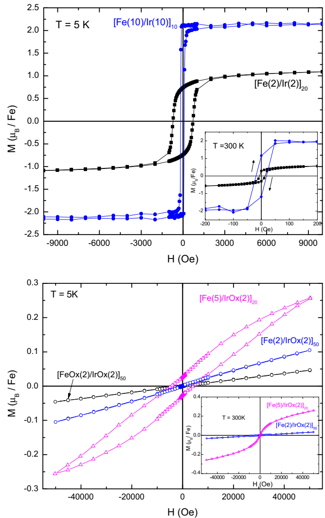
FIG. 8. Magnetic isotherms recorded at T = 5 \text{ K} after field cooling. The insets show the magnetic isotherms recorded at T = 300 \text{ K} .
