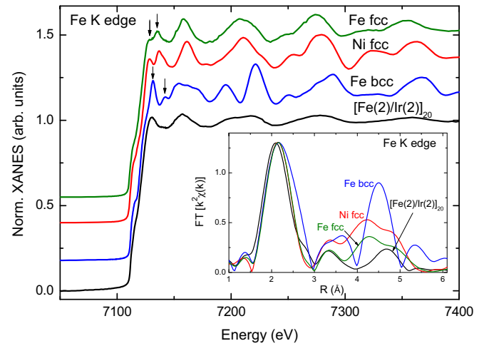
FIG. 2. Fe K-edge XAS spectra recorded on [Fe(2)/Ir(2)] 20 and bulk Fe, bulk Ni, and fcc-Fe nanoparticle [35] references. The inset shows the modulus of the Fourier transforms of the k^2 -weighted EXAFS signals in the range from 3 Å -1 to 10 Å -1 . For the sake of a better comparison the FT of the references has been multiplied by a factor of 0.3.
