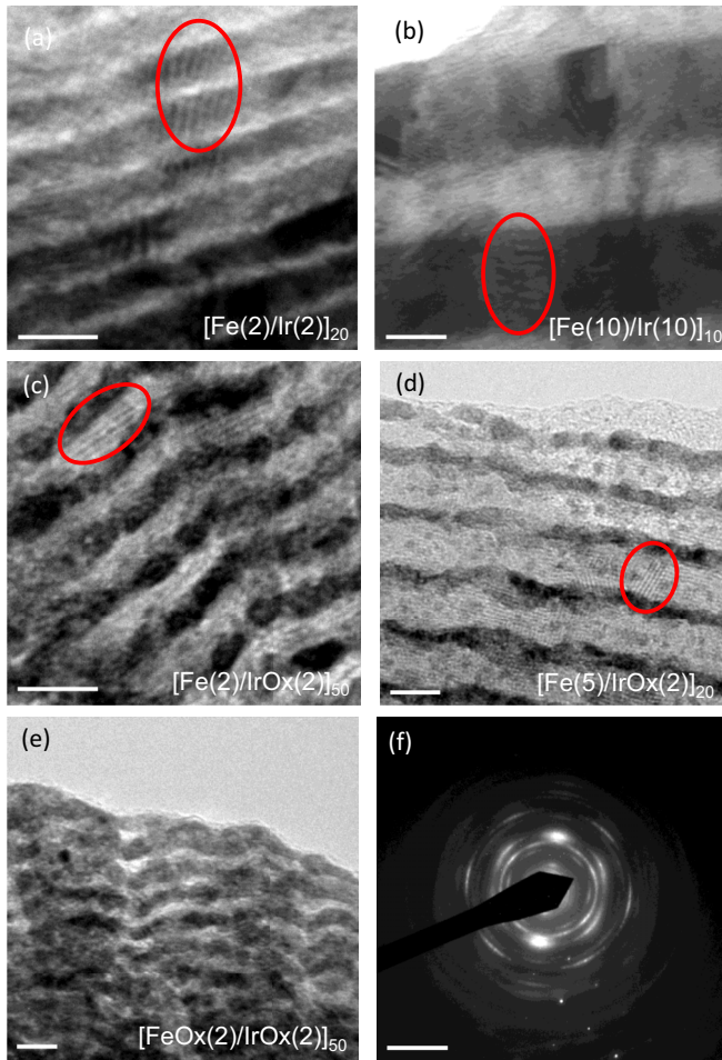
FIG. 1. TEM images of the M/M (top), M/O (middle), and O/O (bottom) samples showing layered structure with darker Ir-containing and lighter Fe-containing layers. Panel (f) shows the FT corresponding to the [Fe(5)/IrOx(2)] 20 sample.
