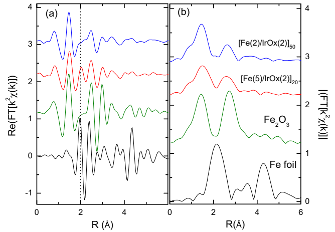
FIG. 6. Fourier transforms [(a) real part, (b) modulus] of the k^2 -weighted Fe K-edge EXAFS signal in the range from 3 \text{ \AA}^{-1} to 10 \text{ \AA}^{-1} . The dotted line is a guide for the eye.
