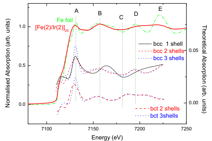
FIG. 3. The Fe K-edge XANES spectra recorded on the [Fe(2)/Ir(2)] 20 sample are compared to the theoretical spectra obtained for Fe bcc clusters.
