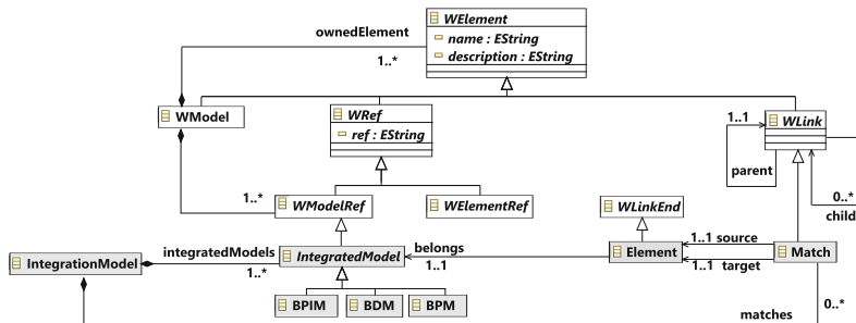
Fig. 6. Integration metamodel
