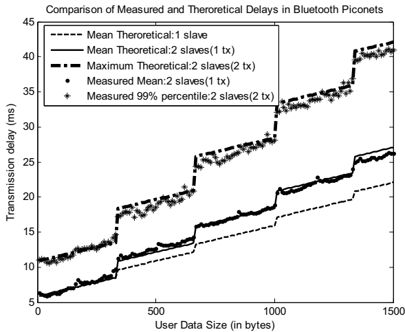
Fig. 4. Comparison of the theoretical model and the measurements of the delay for a piconet of two slaves
