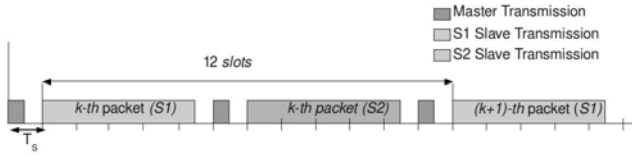
Fig. 2. Time between two consecutive 5-slot packets for a piconet of two slaves when the transmissions of both slaves coincide
