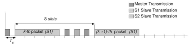
Fig. 1. Minimum time between two consecutive 5-slot packets for a piconet of two slaves when just one slave is transmitting
