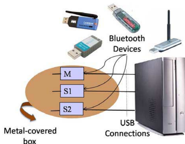
Fig. 3. Testbed for the experiments
