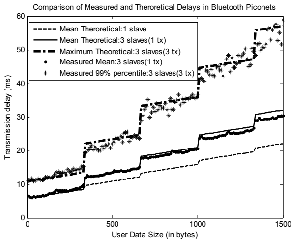
Fig. 5. Comparison of the theoretical model and the measurements of the delay for a piconet of three slaves
