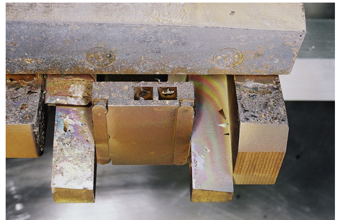
Fig. 50. Photograph of the inner carrier 2IN after removal in 2007. The bottom of Tile 3 is at the top of the picture. Surfaces are covered with a thick deposit, which is showing signs of spalling in certain places. The front face of the mirror test unit is so thickly coated that it is not possible to see where the third channel (with a sample flush to the face) is.
