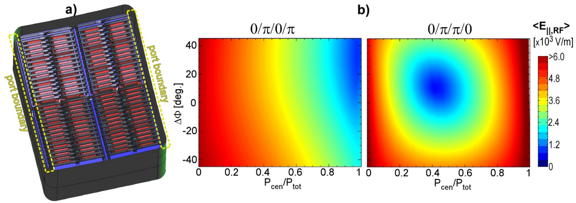
Fig. 10. (a) TOPICA model for the ITER antenna with regions close to PFCs (port boundaries) highlighted; (b) RF feeding diagrams for E_{\parallel,RF} averaged over the regions from (a) ( P_{total} = 1 MW).
