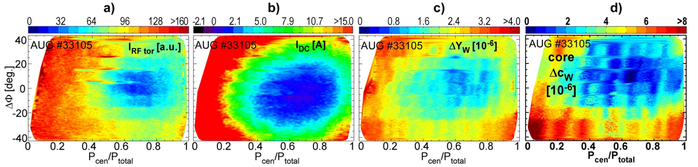
Fig. 5. RF feeding diagrams using strap power balance P_{\text{cen}}/P_{\text{total}} and phase deviation from dipole \Delta\Phi as variables in a discharge with P_{\text{ICRF}} = 1 MW; (a), (b), (c) – local measurements at a single antenna limiter tile (vertical position z \approx 0.2 , left limiter as seen from the plasma) of toroidal RF current I_{\text{rf tor}} (a), DC current circulation I_{\text{DC}} (b) and increment of the W sputtering yield \Delta Y_W (c); d) increment of W content in plasma at T_e \approx 1.5 keV.
