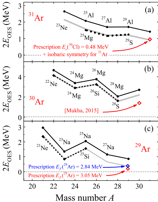
FIG. 14. Odd-even staggering (TES) energies for the isotones leading to ^{31}\text{Ar} (a), ^{30}\text{Ar} (b), and ^{29}\text{Ar} (c) are shown by dashed lines. The OES energies for mirror isobar are given by solid lines. Panel (b) corresponds to Ref. [2]. The solid gray lines are provided to guide the eye. They are shifted down by the constant value of 0.5 MeV, which seems to be the very stable value for variety of isobars and isotones.
