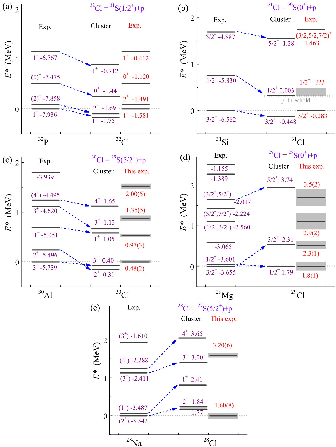
FIG. 13. Energy levels of chlorine isotopes. Vertical axes show excitation energies E^* . The level legend gives spin-parity J^\pi and energies relative to the 1p -emission threshold for the chlorine chain members or 1n -emission threshold for their isobaric mirror partners.
