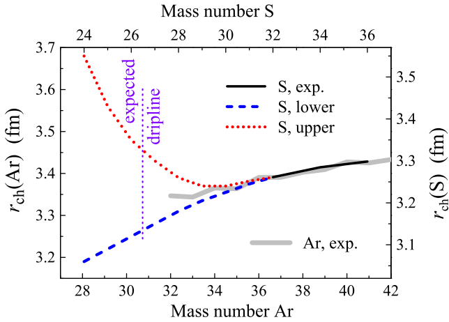
FIG. 12. Charge radii of sulphur isotopes used in the cluster core+ p model for chlorine states. The dependence for sulphur isotopes is aligned with the much better studied dependence for argon isotopes to substantiate the provided extrapolation.
