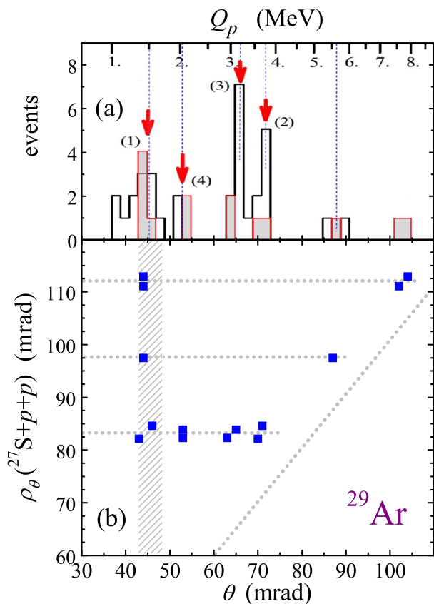
FIG. 6. The angular correlation plot \theta - \rho_\theta (angles are in mrad) for ^{29}\text{Ar} decay via ^{27}\text{S}+p+p channel is shown in (b). The hatched area highlights events from the decay of a ^{27}\text{S}+p resonance assigned as the ^{28}\text{Cl} ground state. The dotted lines guide the eye for the regions corresponding to assumed ^{29}\text{Ar} states. (a) shows the angular correlations \theta_{p-27S} (shaded histogram) obtained as projection on the \theta axis from the ^{27}\text{S}+p+p channel of (b). The \theta_{p-27S} “inclusive” angular correlations obtained from the measured p-^{27}\text{S} coincident events are shown by the black hollow histogram. The labeled (1)–(4) arrows highlight the events inspected for the possible ^{28}\text{Cl} resonance states. The upper axis shows the corresponding 1p -decay energies Q_p . The 45°-tilted dotted line in (b) shows the kinematical limit.
