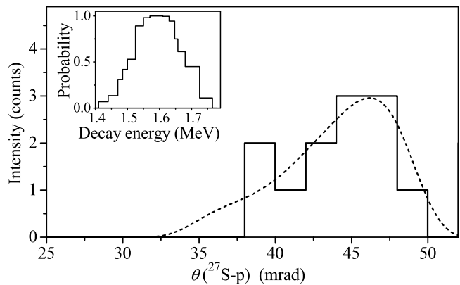
FIG. 7. Best fit of the peak (1) of the \theta_{p-27S} “inclusive” angular correlations from Fig. 6(b) (histogram) by simulations of the setup response to in-flight decays of ^{28}\text{Cl} with the 1p -decay energy of 1.60 MeV (dashed curve). The inset shows probability that the simulated distribution matches the data as function of the 1p -decay energy.
