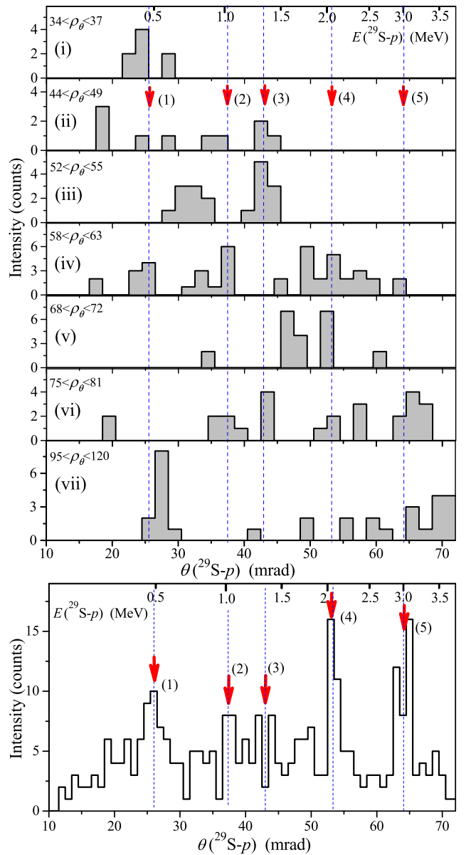
FIG. 10. The “gated” angular correlations \theta_{p-^{29}\text{S}} derived from the measured ^{29}\text{S}+p+p triple-coincidence events, which are selected by choosing the gate conditions within the \rho_\theta ranges corresponding to the highlighted arcs in Fig. 2. The panels (i)–(iv) correspond to the selection gates labeled in Fig. 2 by the same Roman numerals. The additional panels (v)–(vii) present the similar \theta_{p-^{29}\text{S}} correlations selected by the larger \rho_\theta values shown in their upper-left corners. The panel (viii) shows the “inclusive” angular \theta_{p-^{29}\text{S}} correlations obtained from the measured ^{29}\text{S}+p double coincident events (the hollow histogram). The upper axes show the corresponding energies in the ^{29}\text{S}+p system. The arrows (1)–(5) point to the events inspected for possible resonances in ^{30}\text{Cl} as well as the vertical across-panel lines.
