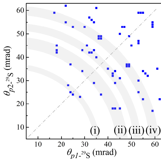
FIG. 2. Angular correlations \theta_{p1-29S} - \theta_{p2-29S} (in mrad) produced from the measured ^{29}\text{S}+p+p coincidence indicating 2p decays of ^{31}\text{Ar} excited states. The shaded arcs labeled by the Roman numerals point to four selected areas where the 2p -decay events have the same decay energy. The data symmetry respective proton permutations is illustrated by the 45^\circ -tilted diagonal dash-dot line.
