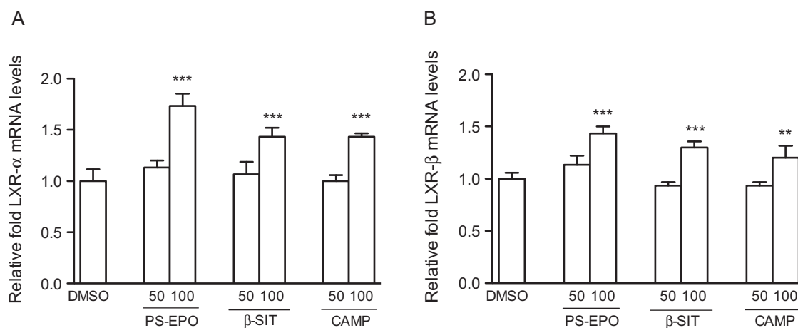
Fig. 3 – Effect of PS-EPO and its main components on LXR mRNA levels in HT-29 cells. Effect of PS-EPO (50 and 100 μg/mL) or β-sitosterol and campesterol (50 and 100 μM) for 48 h on LXR-α gene expression (A) and LXR-β gene expression. (B) The data represent the average median of at least three independent experiments (by triplicate) ± SD. ** P < 0.01 and *** P < 0.001 vs control (DMSO) were determined by one-way analysis of variance followed by Dunnett's test.
