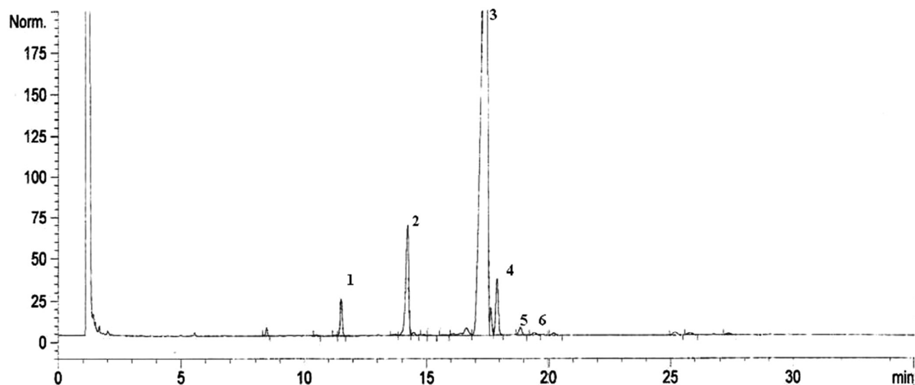
Fig. 1 – Gas chromatogram of the sterols fraction from evening primrose oil. 1. \alpha -Colestanol. 2. Campesterol (9.07%). 3. \beta -Sitosterol (85.34%). 4. Sitostanol (1.42%). 5. \Delta^5 -Avenasterol (3.96%). 6. \Delta^7 -Avenasterol (0.20%).
