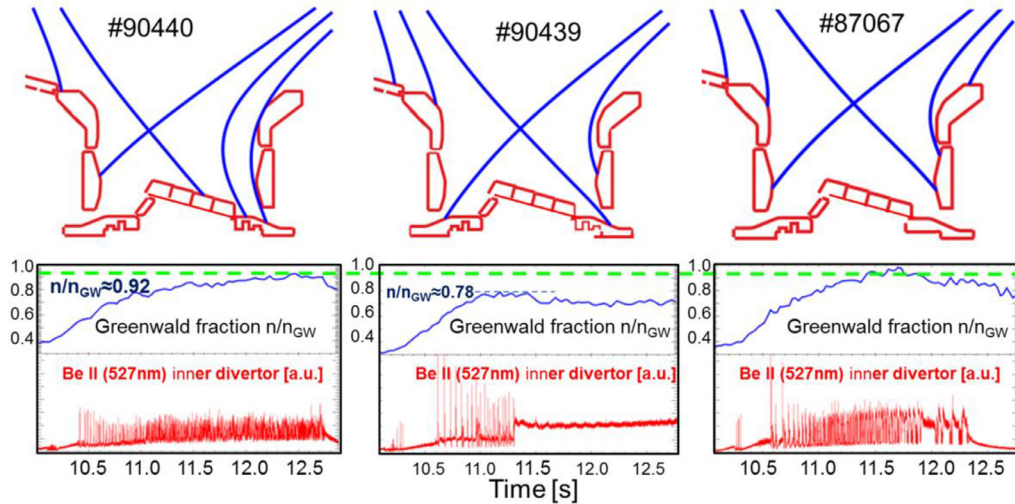
Fig. 13. Evolution of the Greenwald fraction for three discharges with different magnetic shapes.
