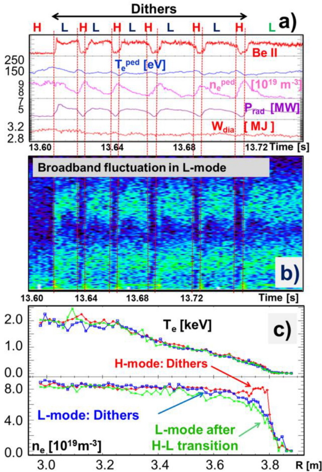
Fig. 4. Characteristic time traces of the high density limit JET-ILW discharges for dithering cycles before the H-L transition: Bell-emission signal, pedestal density n_{ped} and temperature T_{ped} , total radiated power P_{rad} , plasma stored energy W_{dia} as well as power spectrum of a magnetic probe located inside the vessel on the high field side. Also shown n_e and T_e profiles during the transient H-L-H periods.
