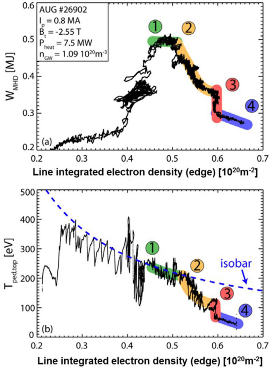
Fig. 6. (a) W_{\text{MHD}} - n_e plot for H-mode DL discharge in AUG; (b) Estimate of the pedestal top temperature plotted versus the edge density. The four phases can also be distinguished, the first phase evolves along an isobaric line. The strong oscillations are caused by heating steps and ELMs. Picture adapted from [11].
