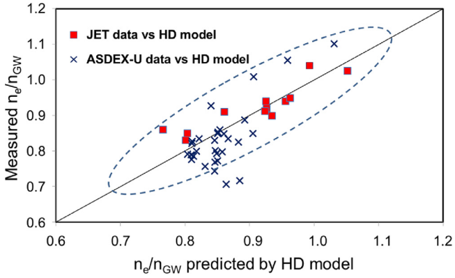
Fig. 14. Experimental measurements of the Greenwald fraction, n_e/n_{GW} , in gas fuelled H-Mode DL discharges in JET-ILW and AUG tokamaks, plotted against the Goldston model [30].
