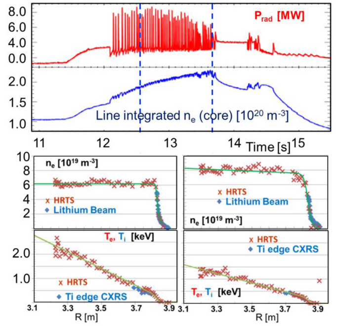
Fig. 7. Time traces of the total radiation and line integrated density (core), the n_e and T_e at two time events during the density ramp in JET-ILW, the long-dashed line mtanh fits to these results.
