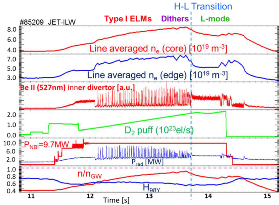
Fig. 1. Time evolution of a typical H-mode density limit discharge on JET-ILW.
