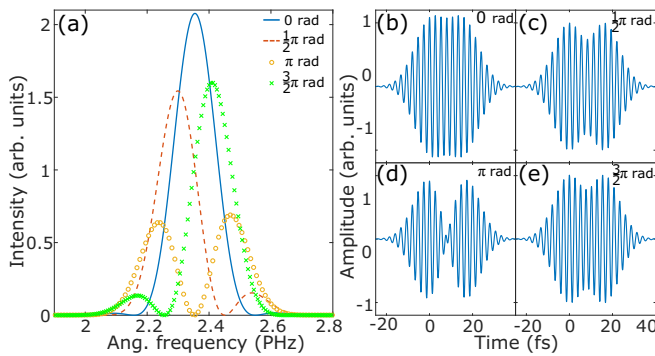
FIG. 2. (a) Spectral intensity and (b)–(e) the corresponding temporal evolution at a fixed delay, but (b) at 0, (c) \pi/2 , (d) \pi , and (e) 3\pi/2 rad relative \varphi_{cep} between the composing pulses of the double-pulse structure. The chosen delay is \tau_d = 16 fs, where the two pulses constructively interfere in the case of 0 rad \varphi_{cep} . The other parameters are the same as those in Fig. 1.
