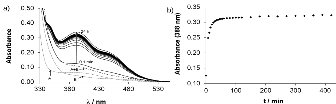
Fig. 3 (a) Time-dependent UV-Vis absorption spectra of the Ru(η 6 -tol)-HQCl-Pro (1:1) system at pH = 3.64 (solid lines). Dotted curves show the absorption spectra of the triaqua organometallic metal ion (A) and HQCl-Pro ligand (B); the dashed curve shows their additive spectrum (A + B). (b) Absorbance values at 388 nm as a function of time. {c([Ru(η 6 -tol)(H 2 O) 3 ] 2+ ) = c(HQCl-Pro) = 101 μM; pH = 3.65; I = 0.20 M (KNO 3 ); T = 25.0 °C; ℓ = 1 cm}.
