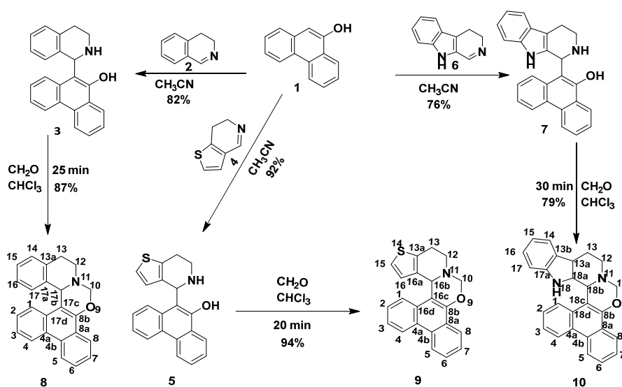
Scheme 1. Syntheses and ring closures of bifunctional compounds 3 , 5 and 7 .
