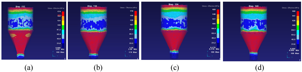
Fig 4: Effective-stress analysis for 90% reduction and \mu = 0.38 (a) square-section (b) hexagonal-section (c) heptagonal-section (d) octagonal-section
