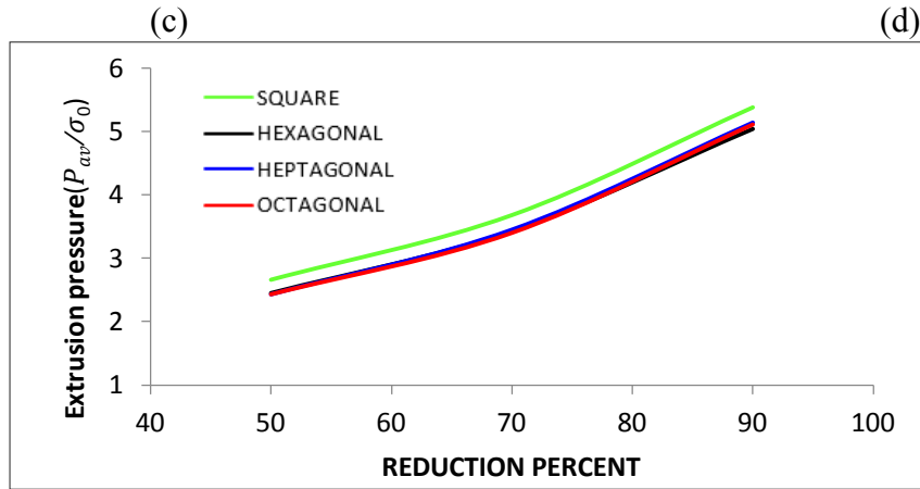
Fig 8: Comparison of (a) predictive load versus punch displacement of different geometry at 50% area reduction (b) predictive load versus punch displacement of different geometry at 70% area reduction (c) predictive load versus punch displacement of different geometry at 90% area reduction (d) Extrusion pressure versus percentage area reduction at ( \mu=0.38 ) (e) Extrusion pressure versus percentage area reduction at ( \mu =0.75 )
