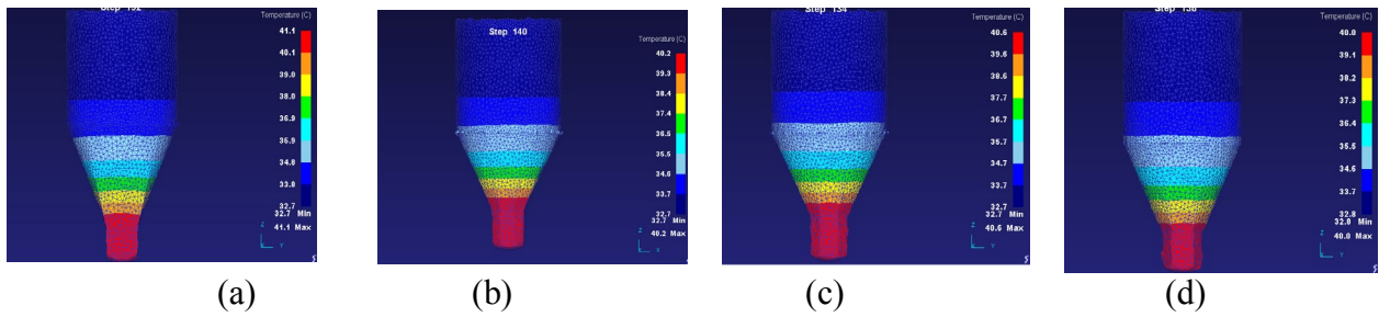
Fig 3: Temperature distribution for 90% reduction and \mu = 0.38 (a) square-section (b) hexagonal-section (c) heptagonal-section (d) octagonal-section
