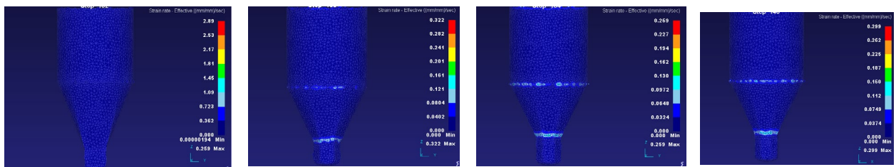
Fig 5: Effective-Strain analysis for 90% reduction and \mu = 0.38 (a) square-section (b) hexagonal-section (c) heptagonal-section (d) octagonal-section
