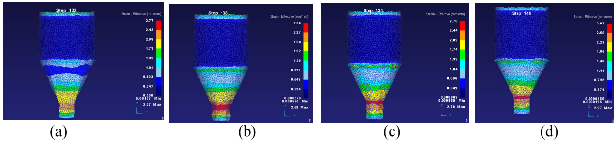
Fig 5: Effective-Strain analysis for 90% reduction and \mu = 0.38 (a) square-section (b) hexagonal-section (c) heptagonal-section (d) octagonal-section
