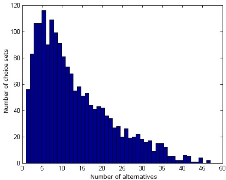
Figure 1: Histogram of |D_n| (50 draws)
