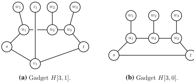
Fig. 2 Examples for variable gadgets
