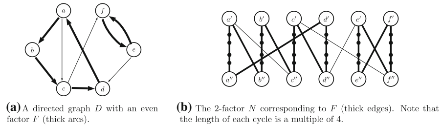
Fig. 4 Reduction from PERFECTEVENFACTOR to C_{4k+2} FREE2FACTOR
