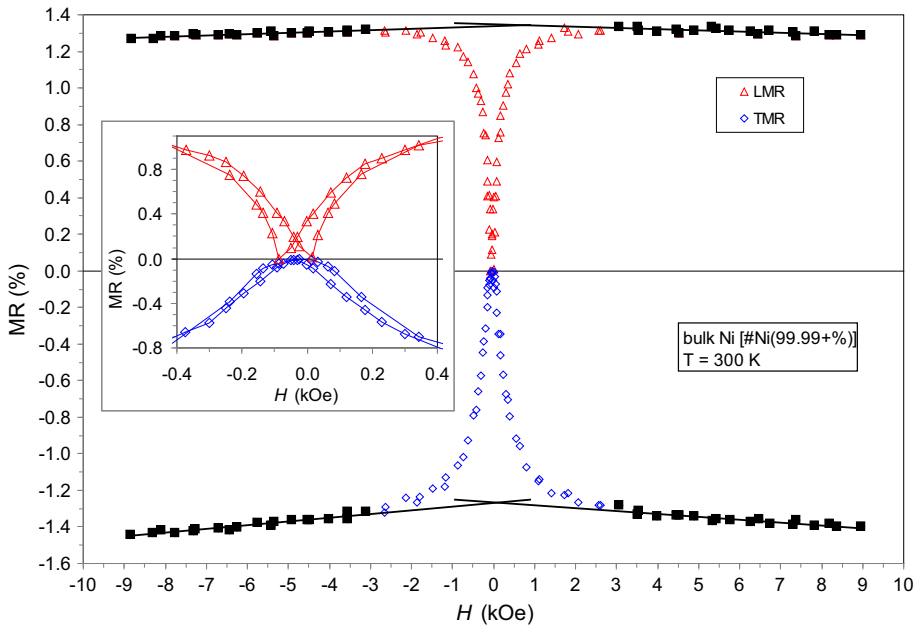
Fig. 1 Room-temperature longitudinal (LMR) and transverse (TMR) MR(H) curves for the bulk Ni foil sample #Ni(99.99+%). The solid squares over the high-field ( |H| \geq 3 kOe) data points indicate data used for a linear fitting and the fit is also indicated (thick solid line). The inset shows a magnified view around zero magnetic field to demonstrate that by the densely measured points around H = 0 , the real maximum and minimum resistivity values were captured. The magnified inset also allows revealing the hysteretic behavior of the magnetoresistance, analogous to the magnetic hysteresis
