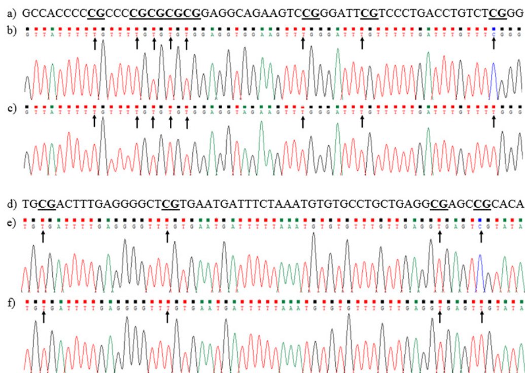
FIGURE 1. Sequence of MSP products. The sequence of (a) AKT1 promoter retrieved from ENSEMBL, (b) methylated CpG site in AKT1 at Chr14: 104796054, and (c) unmethylated CpG site in AKT1 at Chr14: 104796054. The sequence of (d) HTR2A exon-I retrieved from ENSEMBL, (e) methylated CpG site in HTR2A at Chr13: 46896918, and (f) unmethylated CpG site in HTR2A at Chr13: 46896918. The underlined dinucleotides are CpG sites and the arrow shows the cytosine residue after being treated with bisulfite
