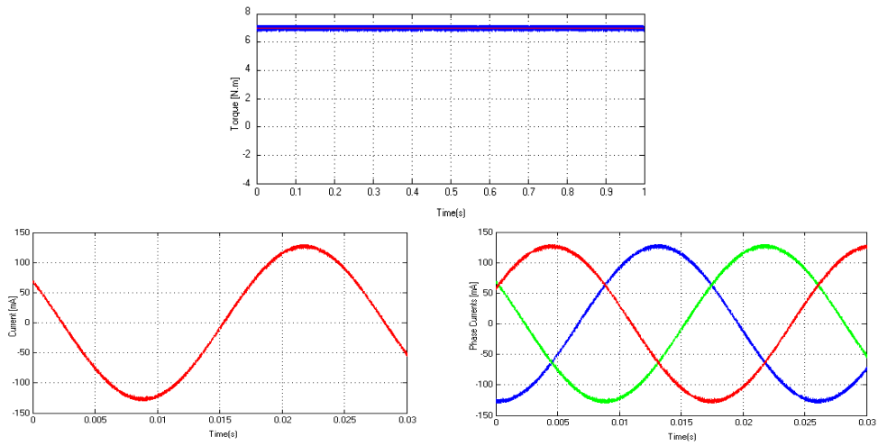
Figure 5. Torque response, phase current and three phase currents of DTC-SVM at 1000 RPM
