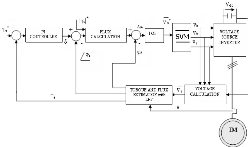
Figure 3. Block scheme of DTC-SVM with Low Pass Filter
