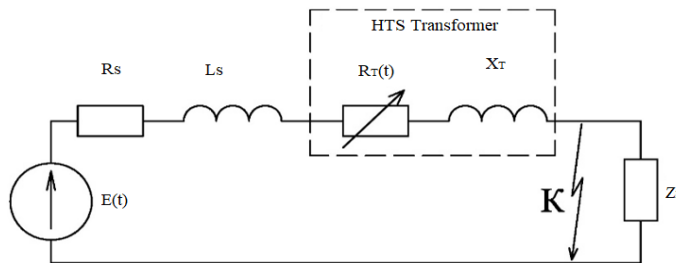
Figure 4. Equivalent circuit for transient process simulation
