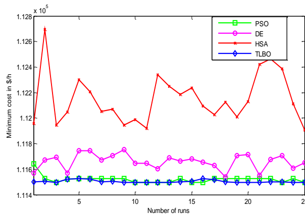
Figure 5. Comparison characteristics of minimum cost obtained for 25 runs
