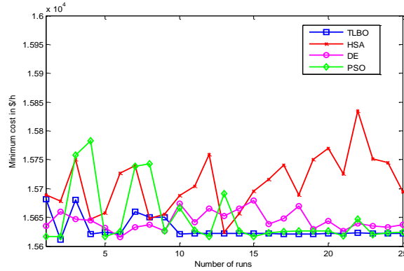
Figure 3. Comparison characteristics of minimum cost Obtained for 25 run
