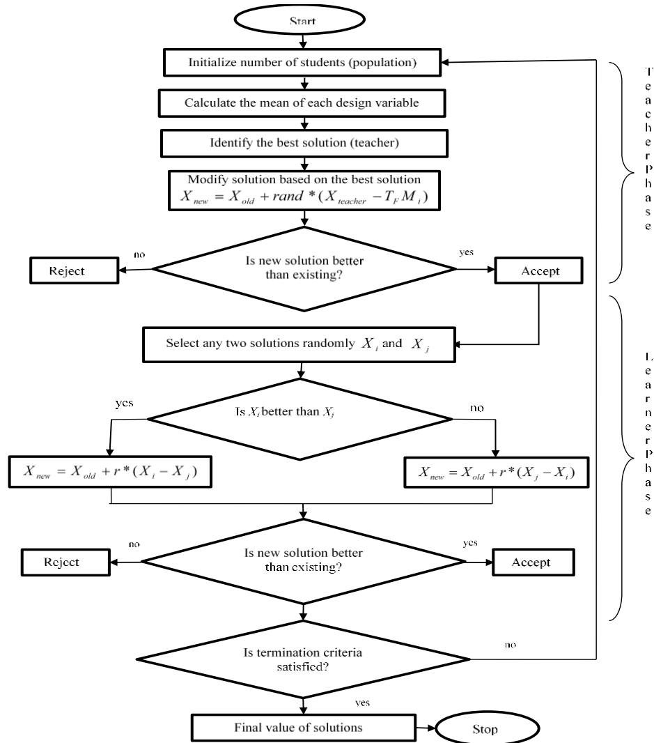
Figure 1. Flow Chart of T & L based optimization algorithm
