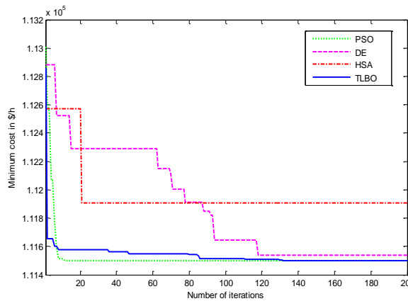
Figure 4. Convergence characteristics of 10-unit system
