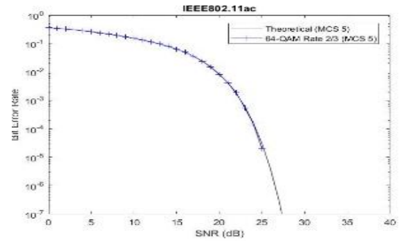
Figure 4(b). Simulation of IEEE 802.11ac with 64 QAM 2/3
