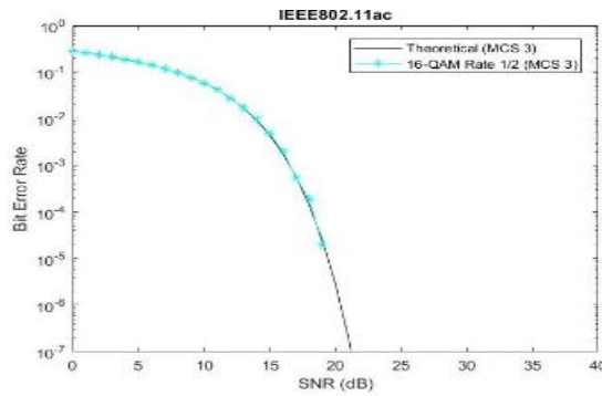
Figure 3(c). Simulation of IEEE802.11 ac with 16 QAM 1/2
