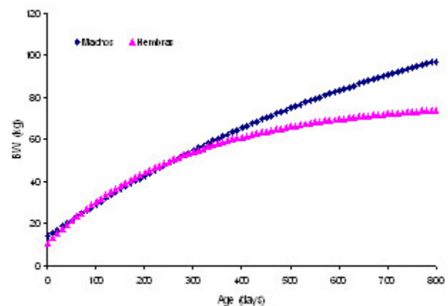
Figure 3. Growth curves for males and females using Brody's model
