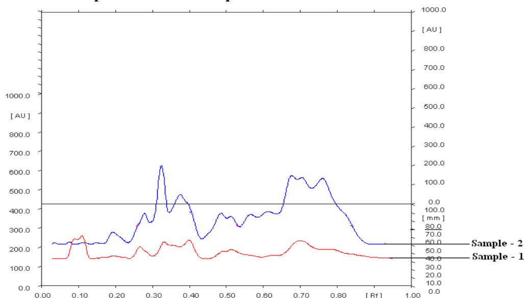
Graph 1: Overview Graph of Sahadevi Extracts At 254nm
