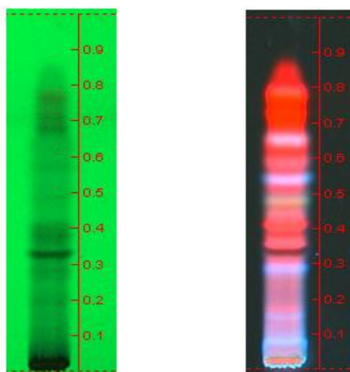
Figure 4: Derivatized TLC Plate Views of Sahadevi Alcoholic Extract AT 254nm AT 366nm AT White Light
