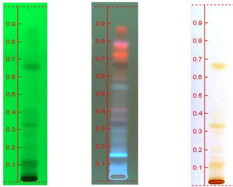
Figure 2: Derivatized TLC plate views of Sahadevi aqueous extract sample
