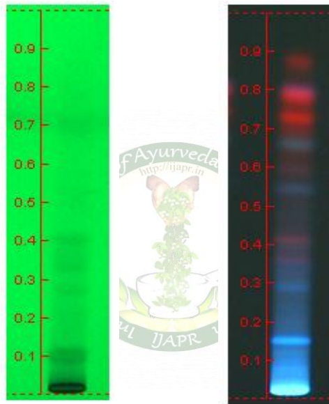
Figure 1: TLC Plate Views of Sahadevi Aqueous Extract Sample
