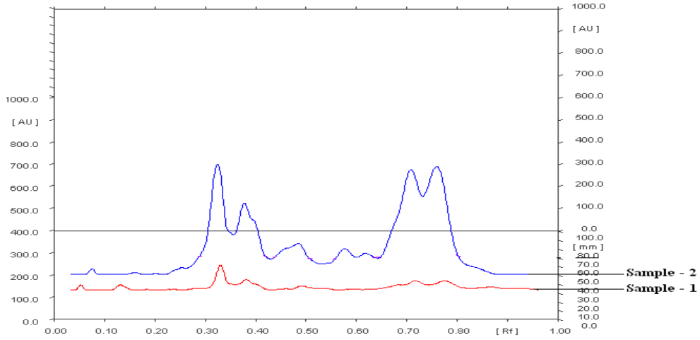
Graph 2: Overview Graph of Sahadevi Extracts at 366nm
