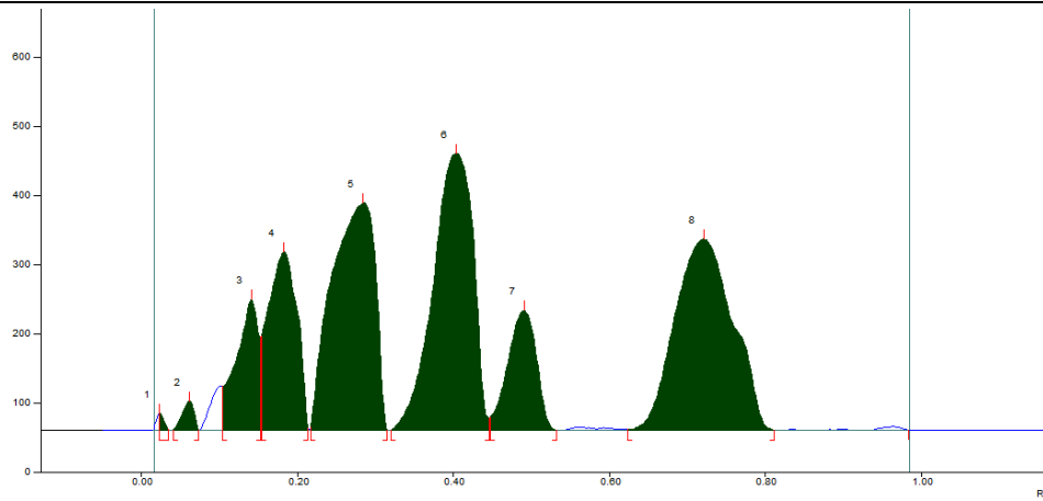
Figure 2. Densitometric scan of the samples at 254 nm
