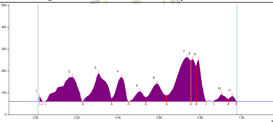
Figure 5. Densitometric scan of the sample at 620 nm
