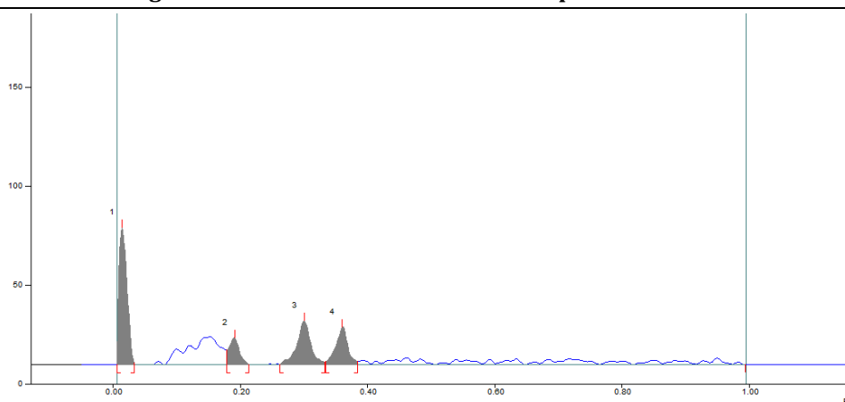
Figure 4. Densitometric scan of the sample at 540 nm
