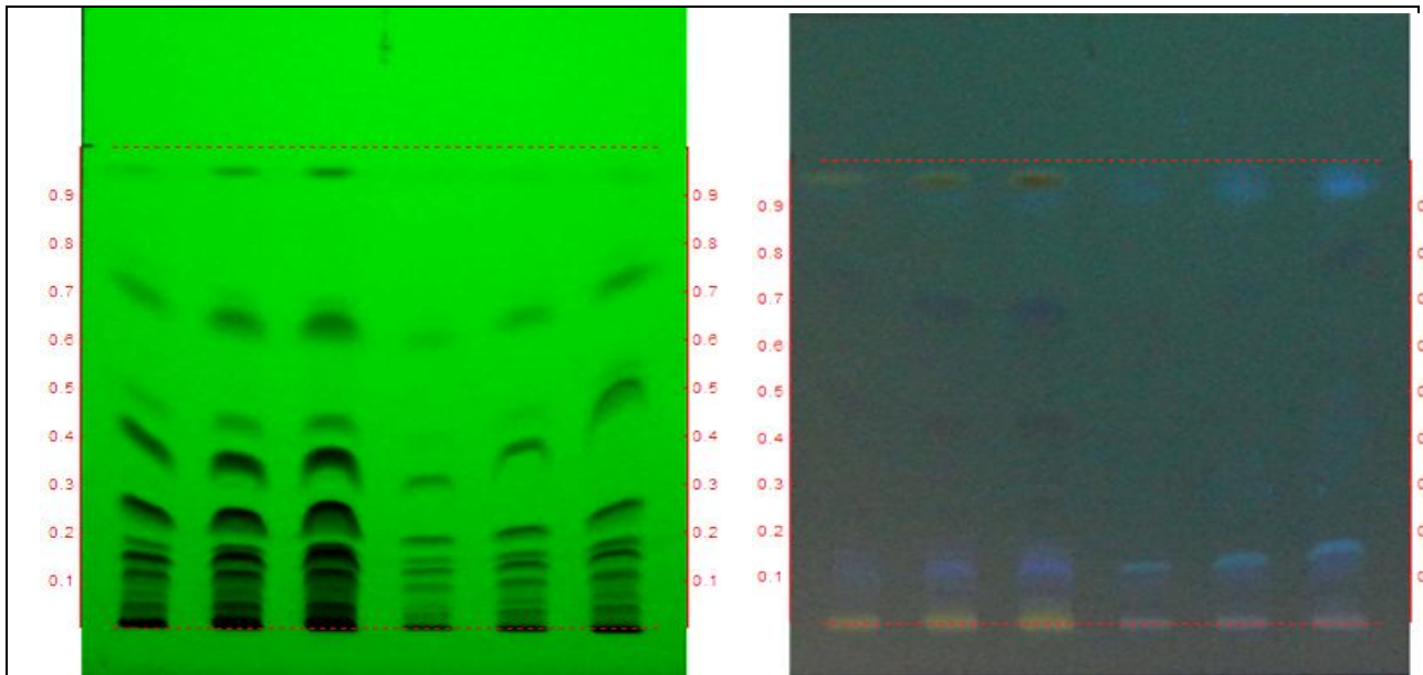
Figure 1. HPTLC photo documentation of Chloroform extract of Jatipatra and Jatiphala
