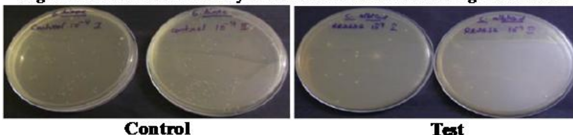
Figure 4: Bactericidal activity of clean hand sanitizer tested against E. hirae
