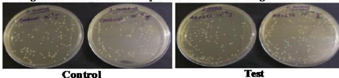
Figure 2: Bactericidal activity of clean hand sanitizer against P. aeruginosa
