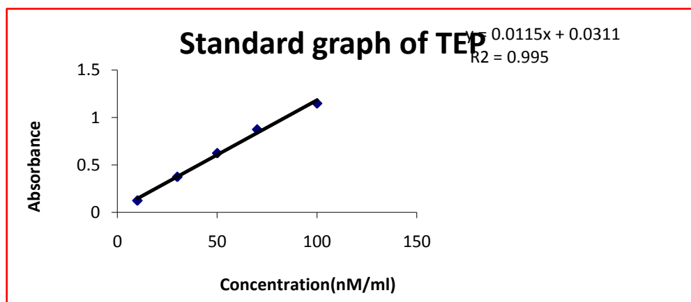
graph of 1, 1, 3, 3-tetra ethoxy propane (TEP)
