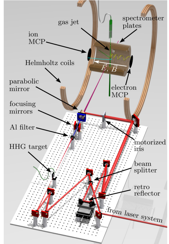
FIG. 3. (Color online) Schematic of the reaction microscope and the interferometer for the generation of mutually delayed XUV pump and IR probe pulses, including a microchannel-plate detector (MCP), an aluminum filter (Al filter), and a high-harmonic-generation target (HHG target). The parallel homogeneous electric and magnetic fields within the spectrometer are represented by the white arrow.
