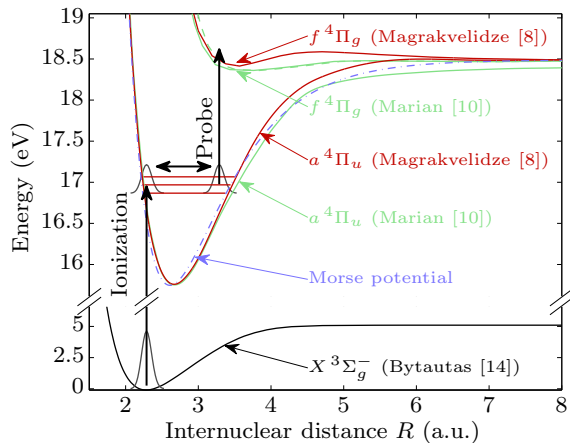
FIG. 2. (Color online) Relevant O_2^+ PECs. The neutral O_2 ground-state potential (black curve) is taken from Ref. [14]. A Morse potential (blue dash-dotted curve) has been adjusted to our experimentally observed quantum-beat frequency and revival time. Relevant vibrational states within this potential are plotted as red horizontal lines. The potentials of the binding a^4\Pi_u state are taken from Refs. [8] (red [dark gray] curve) and [10] (green [light gray] curve). Absorption of a single IR photon transfers population to the repulsive O_2^+(f^4\Pi_g) state taken from Refs. [8] (red [dark gray] curve) and [10] (green [light gray] curve). The dashed green curve is the latter curve shifted by 0.08 a.u. towards larger internuclear distances.
