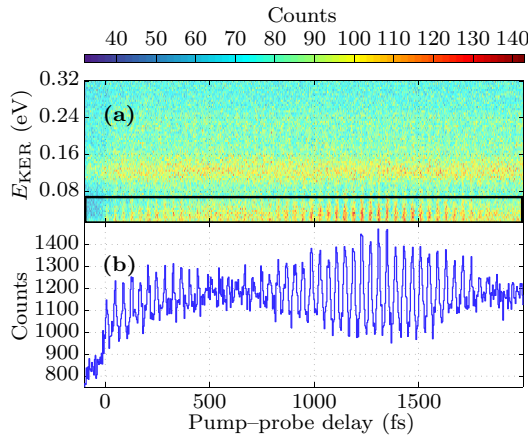
FIG. 4. (Color online) (a) Number of detected O^+ fragments as a function of pump-probe delay and E_{KER} . (b) Projection of events within the black box in panel (a) onto the time-delay axis. For positive delays, the XUV pulse precedes the IR pulse.
