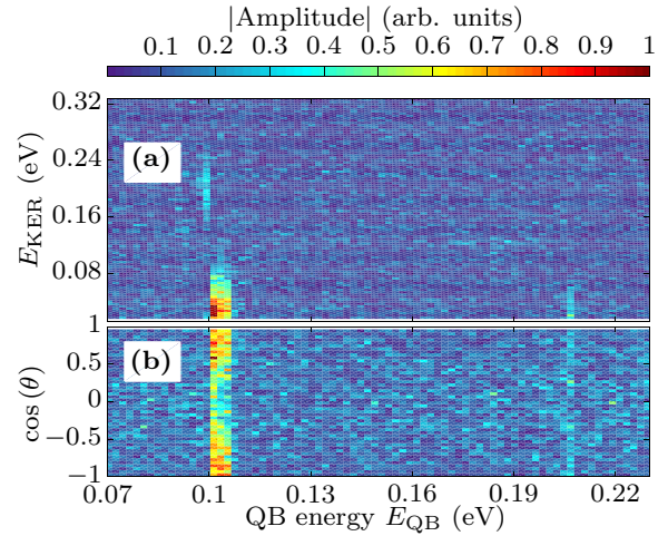
FIG. 5. (Color online) (a) QB spectrum of the data shown in Fig. 4(a). The distinct lines in the QB energy result from the oscillatory behavior of the O^+ yield as a function of the time delay. (b) Amplitude of the Fourier transform of the delay-dependent yield of low energetic O^+ ions as a function of \cos(\theta) . The angle \theta designates the orientation of the molecular axis relative to the identical linear polarization directions of the XUV and IR pulses.
