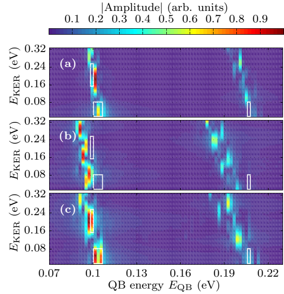
FIG. 7. (Color online) QB spectra of the simulated O^+ yield as a function of E_{KER} . (a) Obtained by using the binding O_2^+(a^4\Pi_u) potential from Ref. [8] (red [dark gray] curve in Fig. 2) and the repulsive O_2^+(f^4\Pi_g) PEC adapted from Ref. [10] (green [light gray] dashed curve in Fig. 2). (b) Obtained by using the binding a^4\Pi_u and the repulsive f^4\Pi_g PECs from Ref. [10] (green [light gray] solid curves in Fig. 2). (c) Obtained by using a Morse potential (blue dash-dotted curve in Fig. 2) and the repulsive f^4\Pi_g PEC adapted from Ref. [10] (green [light gray] dashed curve in Fig. 2).
