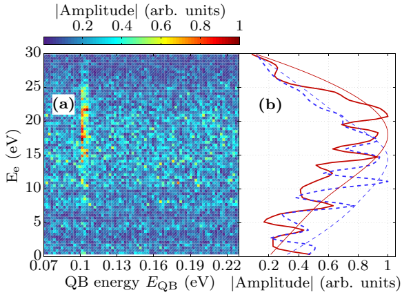
FIG. 8. (Color online) (a) QB spectrum of photoelectrons measured in coincidence with low energetic O^+ . Plotted is the Fourier amplitude as a function of the QB energy and the photoelectron kinetic energy E_e . (b) Red bold curve: Projection of the QB signal at E_{QB} \approx 0.1 eV shown in panel (a) onto the E_e axis. Blue bold dashed curve: Projection of the dc component at E_{QB} < 0.005 eV onto the E_e axis. For better comparison the curves in panel (b) are smoothed and normalized. In addition schematic envelopes of the spectra are shown (thin red solid curve and blue dashed curve).
