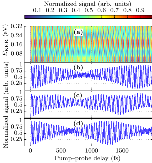
FIG. 6. (Color online) Simulated yield of O^+ fragments as a function of pump-probe delay obtained with a coupled-channel simulation involving different sets of PECs. (a) Yield as a function of pump-probe delay and E_{KER} using the binding O_2^+(a^4\Pi_u) potential from Ref. [8] (red [dark gray] curve in Fig. 2) and the repulsive O_2^+(f^4\Pi_g) PEC adapted from Ref. [10] (green [light gray] dashed curve in Fig. 2). (b) Projection of the lower E_{KER} band in panel (a) onto the time-delay axis. (c) Same as panel (b) but for the binding a^4\Pi_u and the repulsive f^4\Pi_g PECs from Ref. [10] (green [light gray] solid curves in Fig. 2). (d) Same as (b) but using a Morse potential (blue dash-dotted curve in Fig. 2) and the repulsive f^4\Pi_g PEC adapted from Ref. [10] (green [light gray] dashed curve in Fig. 2).
