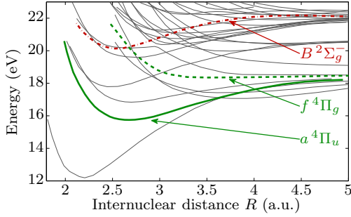
FIG. 1. (Color online) Selection of O_2^+ PECs from Ref. [10]. We consider (i) a vibrational wave packet that oscillates within the O_2^+(a^4\Pi_u) potential (bold green solid curve) and is probed to the O_2^+(f^4\Pi_g) PEC (bold green dashed curve) and (ii) predissociation out of the O_2^+(B^2\Sigma_g^-) state (bold red dash-dotted curve).
