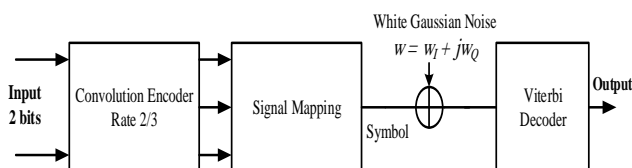
Figure 3: Trellis coded modulation model for coded 8PSK signal
