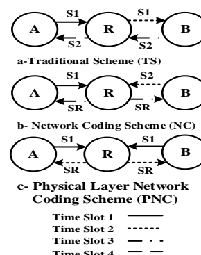
Figure 1: Transmission schemes for the two way relay channels
