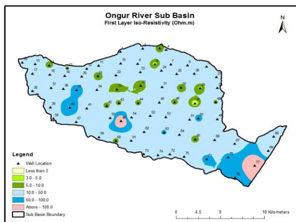
Fig. 3 First Layer Isoresistivity Map
